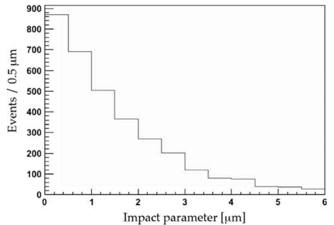
Fig. 5. Impact parameter resolution with a 20 μm stainless steel window.
