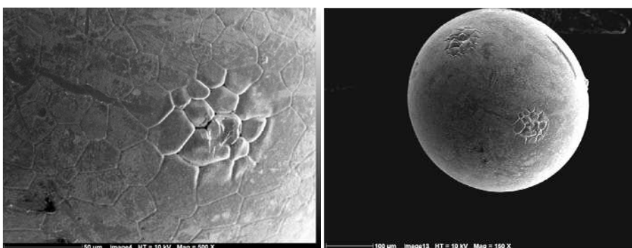
Figure 2 : SEM pictures of the surface of a \text{UO}_2 particle corroded in open to air atmosphere.
