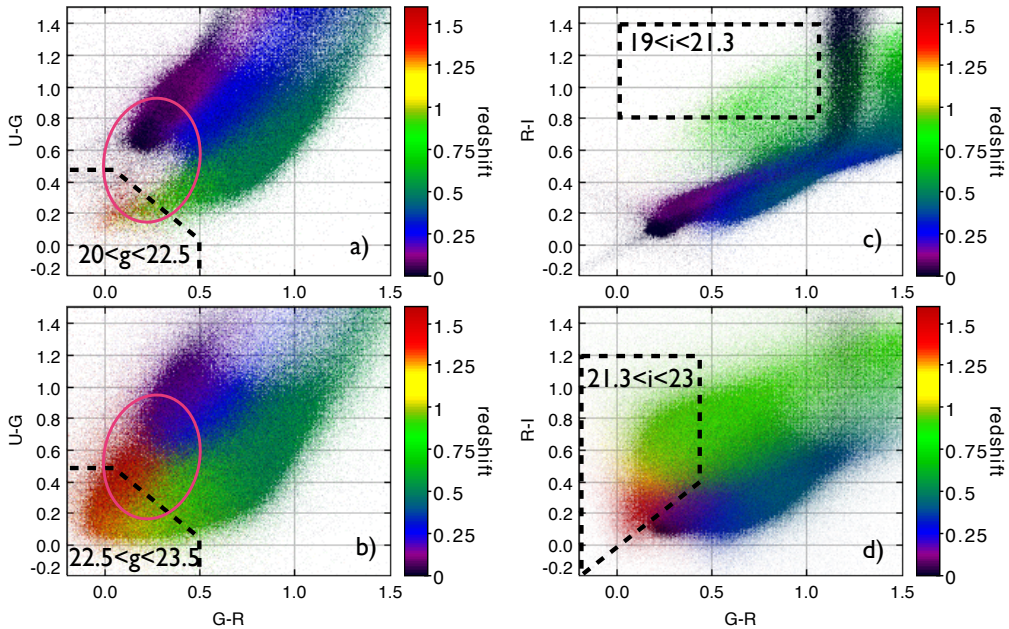
Fig. 2. Color-color diagrams in the CFHTLS photometric database. Left: The ugr selection for the bright (top) and the faint (bottom) samples. Right: The gri selection for the bright (top) and the faint (bottom) samples.
