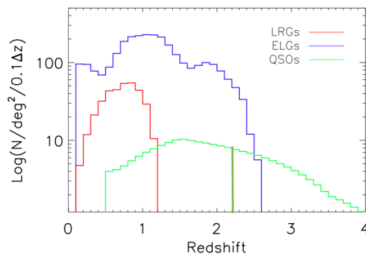
Fig. 1. n(z) distribution for targets selected for BigBOSS (courtesy of Nick Mostek, BigBOSS collaboration).
