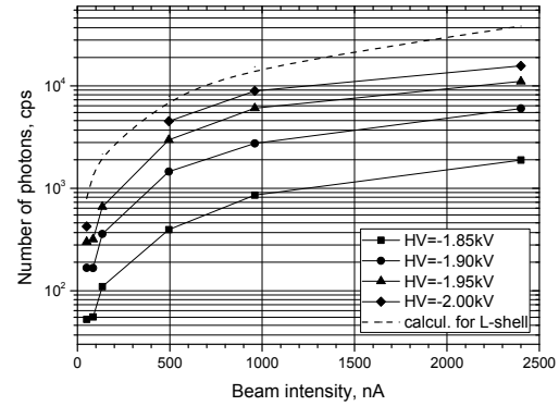
Figure 4: Comparison of count rates for different values intensities and applied voltage. Theoretical estimation of count rate due L-shell ionisation is presented.
