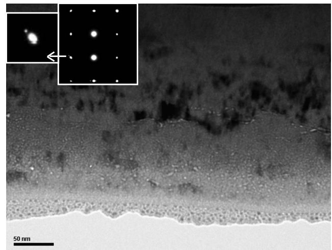
FIG. 8. Under focus TEM micrograph recorded in off-Bragg condition on a cross section of YSZ implanted with 5 \times 10^{16} cm ^{-2} Cs ions at 900 °C.
