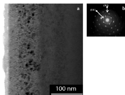
FIG. 5. (a) Bright-field underfocus TEM micrograph of YSZ implanted with 300 keV Cs ions ( 5 \times 10^{16} \text{ cm}^{-2} ) and annealed at 750 °C during 1 h. Recrystallization occurs by the formation of rounded nanocrystals. Between crystallites, cavities are visible in this underfocused image. Note that in off-Bragg conditions, the contrasts of distorted domains created in the deeper crystalline damaged zone are not visible here but they are present as these defects are not annealed at this temperature. (b) Diffraction pattern corresponding to the TEM image. Non epitaxial recrystallization is associated with the apparition of rings corresponding to the YSZ lattice parameters.
