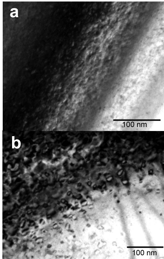
FIG. 6. Bright-field TEM micrographs of YSZ implanted in situ with 70 keV Cs ions ( 3 \times 10^{14} cm ^{-2} , 0.9 dpa) (a) at RT and (b) at 750 °C. Images were recorded in Bragg conditions using g=111 .
