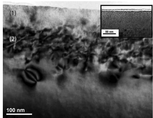
FIG. 7. Bright-field TEM micrographs of YSZ implanted with 300 keV Cs ions ( 1 \times 10^{16} cm ^{-2} ) at 900 °C. The general view shows the overall damaged zone with two beam dynamical conditions. In inset is presented, with the same space scale, the subsurface layer recorded with off-Bragg and underfocus image conditions showing the presence of bubbles.
