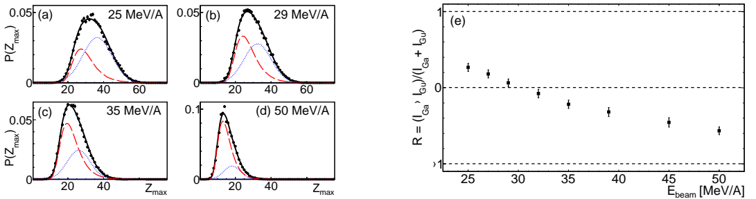
Figure 2. (Color online) Analysis of ^{129}\text{Xe} + \text{nat}\text{Sn} experimental data: (a-d) largest fragment charge distributions, (Black solid curve) best fit to the data using eq. (1), (Red dashed curve) Gumbel component, (Blue dotted curve) Gaussian component; and (e) evolution of the relative weight between the two components, as a function of the beam energy.
