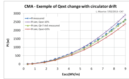
Figure 11: Effect of the circulator thermal drift on the cavity Q ext .
