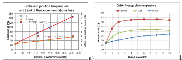
Figure 8: Operating temperatures.
