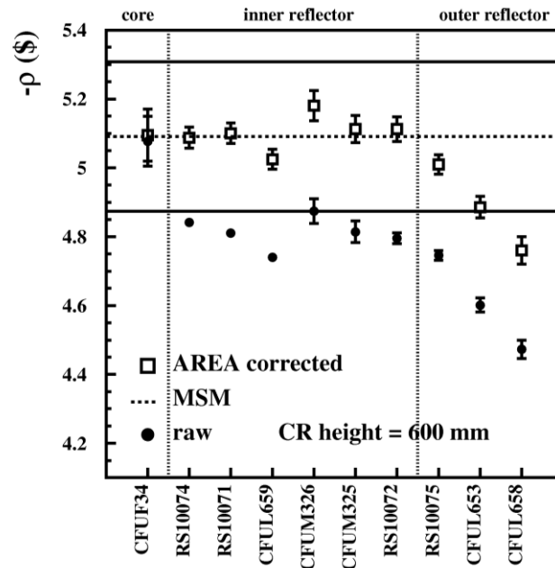
Figure 4. Uncorrected (solid dots) and corrected (open squares) reactivity values extracted from detector counts for the reactor configuration SC1/CR=600 mm. The MSM reference value is the dashed line and its uncertainty range is given by the solid lines.
