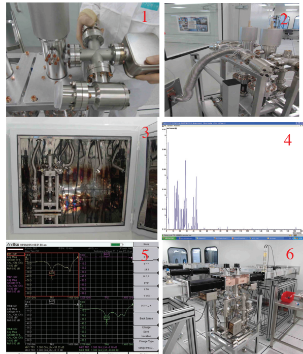
Figure 4: (1) Pumping group mounting, (2) Leak check, (3) In-situ baking, (4) RGA spectrum record, (5) Antenna tuning, (6) installation in RF test bench.
