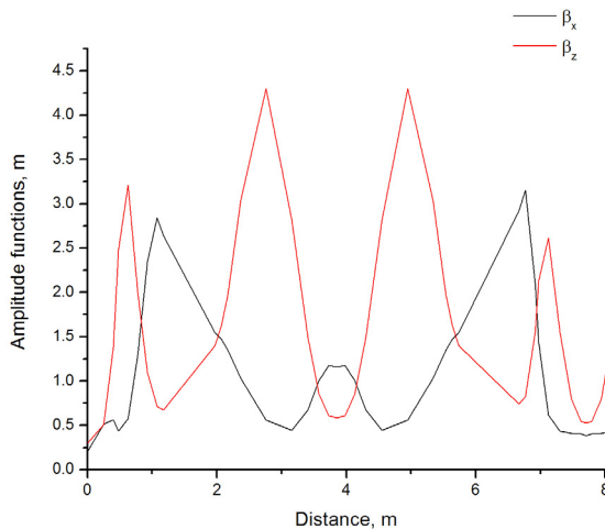
Figure 3: The beta functions of modified lattice.
