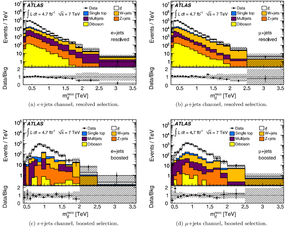
FIG. 9 (color online). The t\bar{t} invariant mass spectra for the two channels and the two selection methods. The shaded area indicates the total systematic uncertainties.
