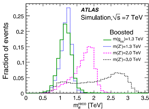
(b) Boosted reconstruction.
