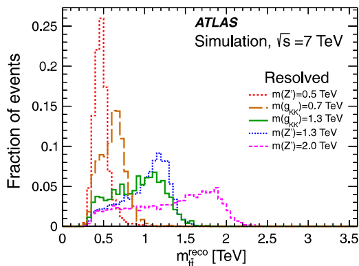
(a) Resolved reconstruction.
