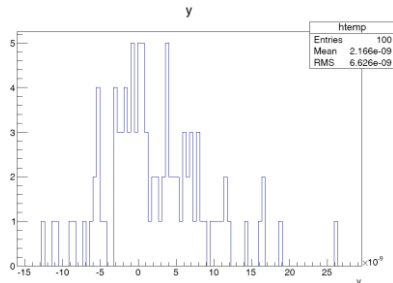
Figure 5: Orthogonality check of \alpha_x knob when introducing roll errors 800 \mu rad.
