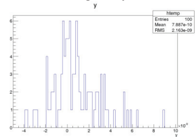
Figure 4: Orthogonality check of \alpha_x knob when introducing roll errors 300 \mu rad.
