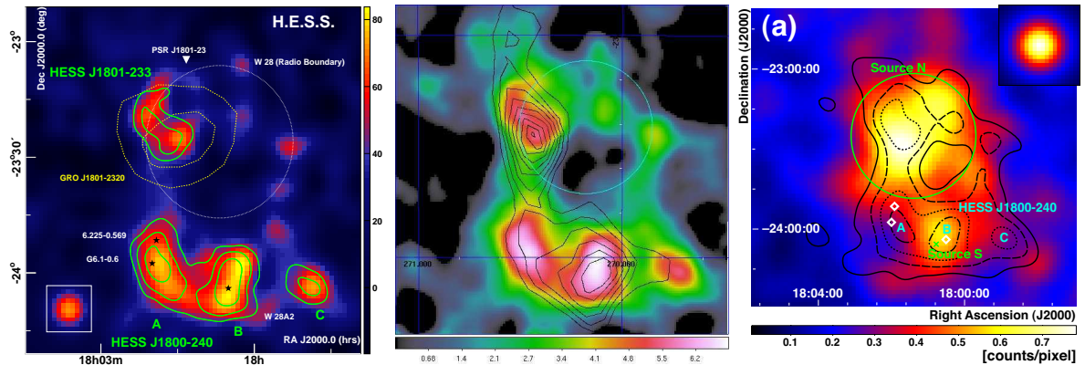
Figure 1: The GeV-TeV picture of the W28 field. The position of the supernova remnant is indicated by a white or green circle. Left: The VHE gamma-ray excess map seen by H.E.S.S. Middle: The HE gamma-ray excess contours from Agile in black over-imposed on the H.E.S.S. excess map. Right: The HE gamma-ray excess map from Fermi-LAT with the H.E.S.S. excess contours overlaid as black lines.
