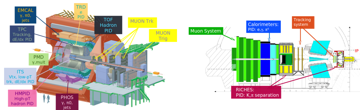
Figure 1: The geometry of the Alice (left) and LHCb (right) detectors. The sub-detectors contributing to the particle identification and described in this paper are indicated.
