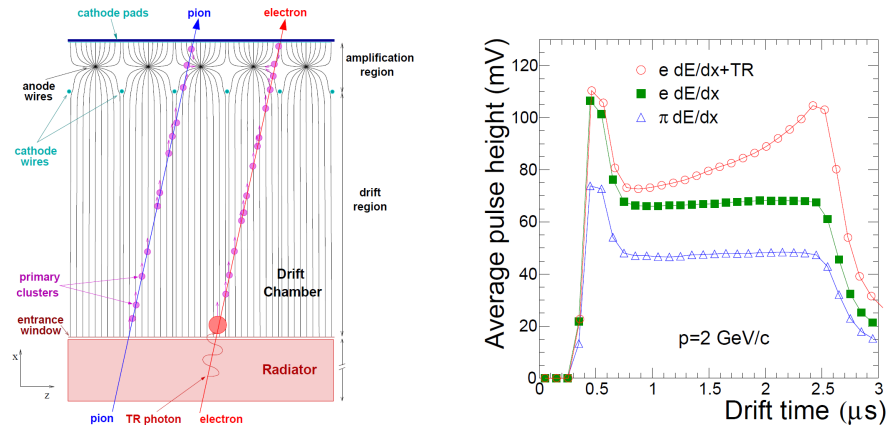
Figure 5: Drawing of a transition radiation detector layer (left) and comparison of the signal seen by the detector with and without TRD for electrons and \pi . The after-pulse for electrons with TRD is clearly visible for a drift time of \sim 2.5\mu\text{s}
