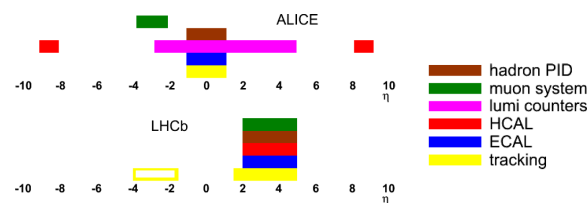
Figure 2: Rapidity regions covered by the Alice (top) and LHCb (bottom) experiments and by some of the sub-detectors used for particle identification.
