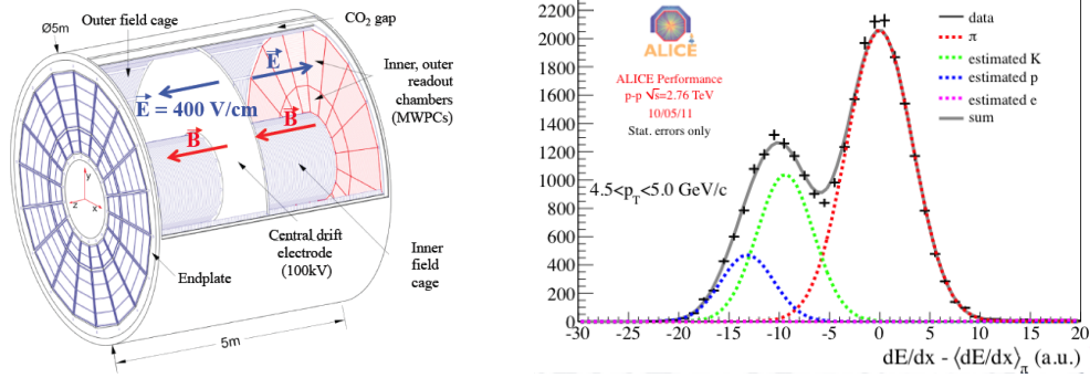
Figure 4: Schematics of the Alice large TPC (left) and \pi , K , proton, electron dE/dx with respect to average \pi dE/dx superimposed with data points.
