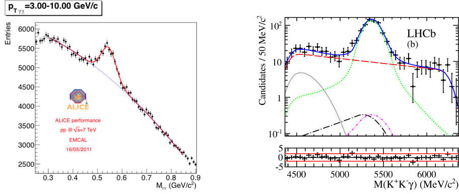
Figure 8: Left: \gamma\gamma invariant mass from the EMCAL calorimeter of Alice and reconstruction of the \eta particle. Right: B_s^0 meson invariant mass reconstruction for the B_s^0 \rightarrow \phi\gamma decay with LHCb (the green dotted-line is the fitted signal contribution). The resolution (rms width) on the B is \sim 92 \text{ MeV}/c^2 and is mostly related to the calorimeter resolution.
