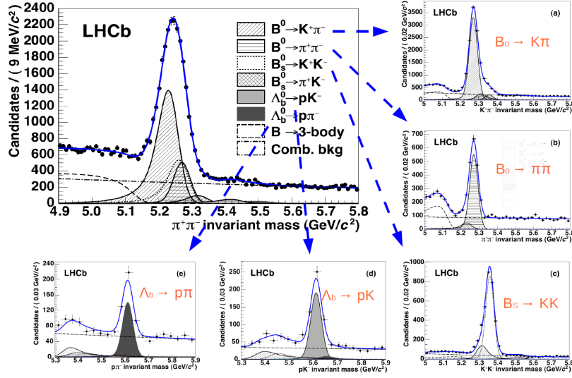
Figure 7: The large top-left plot shows two-body B meson and \Lambda_b hadronic decays reconstructed by LHCb when the two particles are interpreted as charged pions; no particle identification is used here. The separation into exclusive decay subsamples ( B^0 \rightarrow K\pi (a), B^0 \rightarrow \pi\pi (b), B_s^0 \rightarrow KK (c), \Lambda_b \rightarrow pK (d) and \Lambda_b \rightarrow p\pi (e)), based on the RICH identification of the daughter particles leads to the production of sets of candidates with a large efficiency and a low pollution, the mother particle peak being clearly visible.
