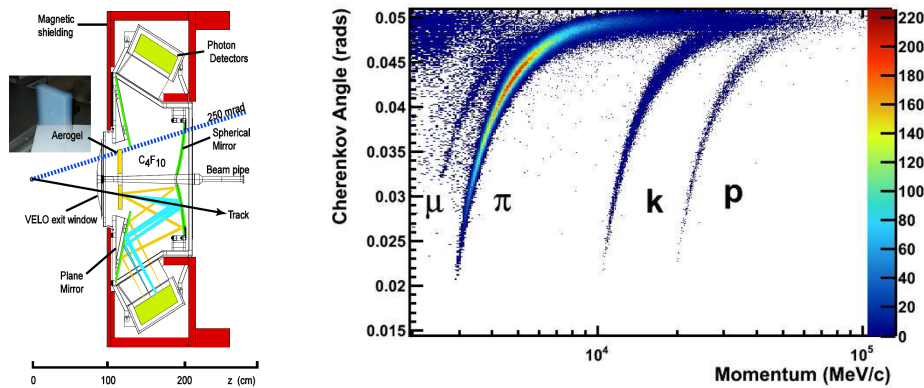
Figure 6: Schematics of the RICH-1 detector of LHCb (left). The two media producing cones are aerogel and C_4F_{10} . Mirrors extract the light towards the HPD located into magnetic field shielding boxes. The right plot shows the separation among several particle species from CF_4 (RICH-2).
