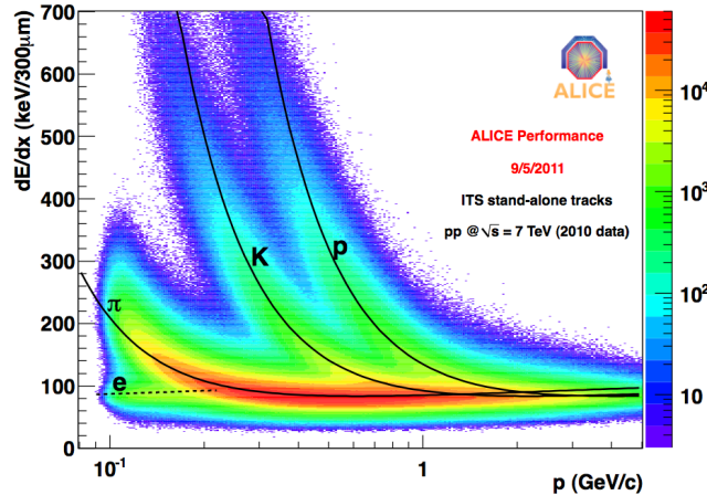
Figure 3: dE/dx measured in the ITS as a function of the particle momentum.
