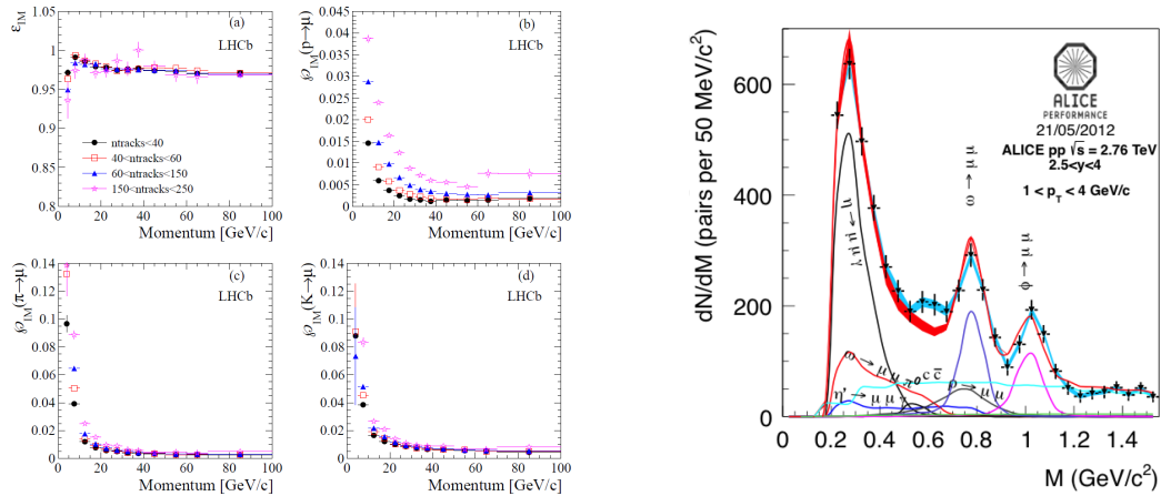
Figure 9: LHCb muon spectrometer efficiency (a) and misidentification rates (b, c and d) as a function of the particle momentum (left). The right plot shows the reconstruction of the invariant mass of resonances built from muon pairs in Alice.
