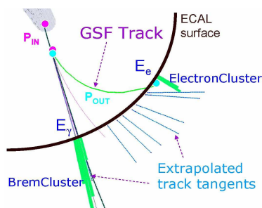
FIGURE 2: Particle-flow clustering
