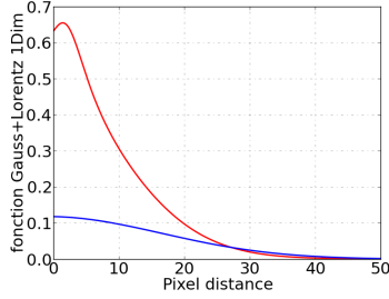
FIGURE 5: Distribution gauss+lorentz
