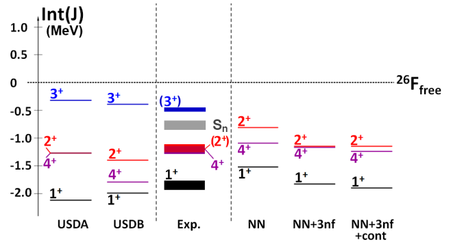
FIG. 3: (Color online) Calculated and experimental interaction energies \text{Int}(J) in MeV in ^{26}\text{F} . Shell-model calculations are shown in the first column using the USDA or USDB interactions, while the third column shows results obtained with CC calculations. Experimental results are in the center. The thickness of the lines corresponds to \pm 1\sigma error bar.
