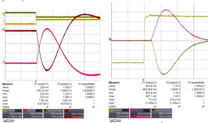
Fig. 9. Screenshot of the response of a complete chain to P and N polarities. In (a) is shown the CSA+slow shaper and in (b) CSA+fast shaper.
