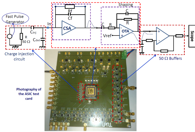
Fig. 8. Test setup and photo of the test board supporting the ASIC (device under test). On the top, is shown a synoptic of the test board.
