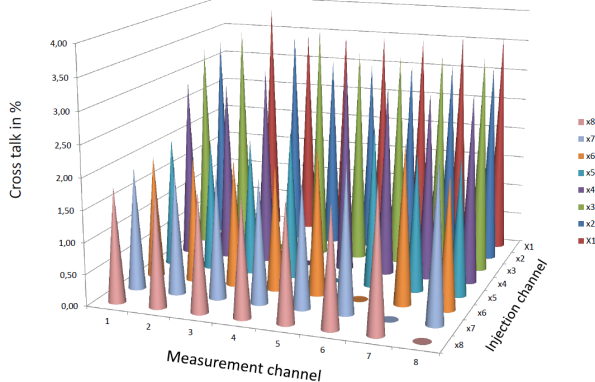
Fig. 13. Crosstalk between the CSA+Slow shaper channels measured for the electron configuration.
