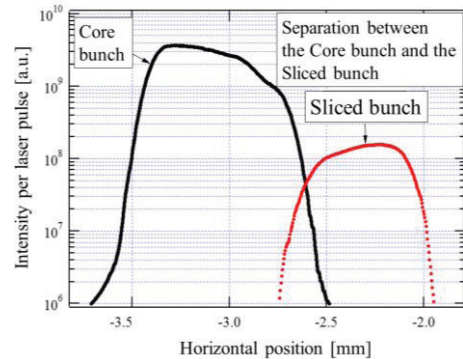
Figure 7: Intensity of the core bunches and sliced bunches in the CRISTAL versus the horizontal position.
