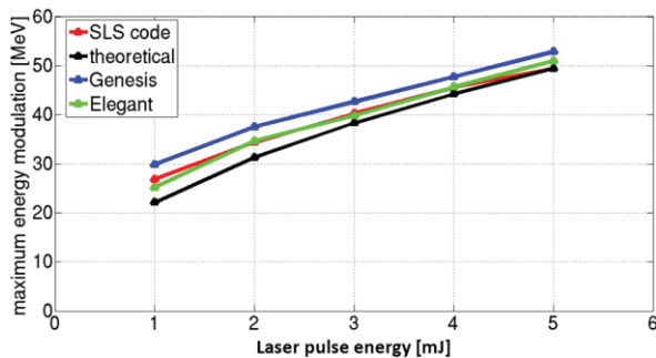
Figure 4: Maximum energy modulation calculated with the SLS code, ELEGANT, GENESIS and the analytical expression (theoretical).
