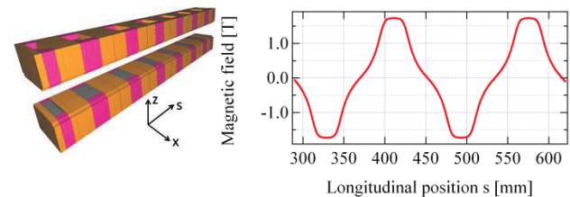
Figure 1: RADIA Short model of three periods (left) and calculated magnetic field at minimum gap (14.5 mm).
