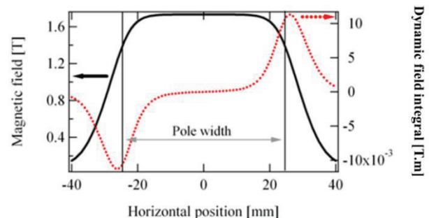
Figure 2: Transverse variation of the field (—) at minimum gap and Dynamic Field Integral (...).
