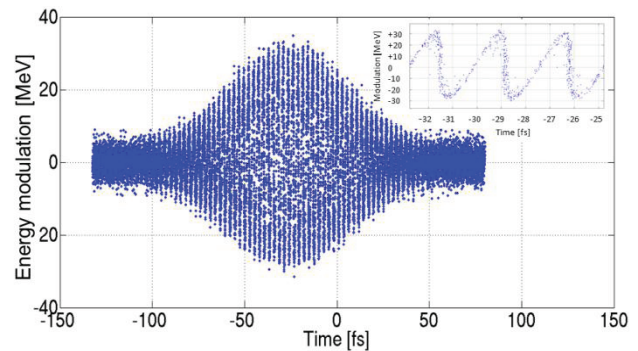
Figure 5: Energy modulation of electrons at the exit of the modulator W164.
