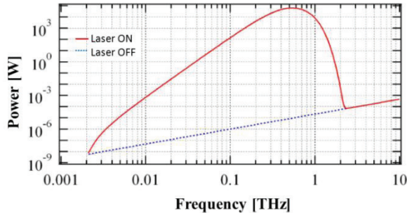
Figure 6: Calculated power radiated by the AILES dipole at 500 mA during Slicing operation (Laser ON) and user operation (Laser OFF). The energy modulation is set to 14 MeV. The laser pulse width is 50 fs.
