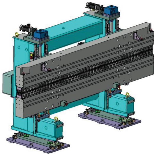
Figure 3: Carriage of the modulator (left) and half-period support equipped with magnets and poles (right).
