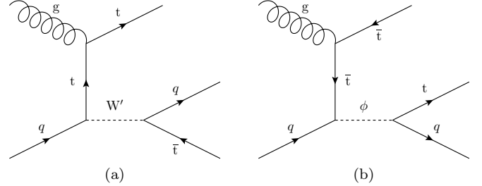
FIG. 1: Example production and decay Feynman diagrams for the (a) W' and (b) \phi models.
