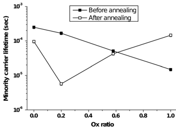
Figure 12: Evolution of minority carrier lifetime for different SiN and SiON layers according to the Ox ratio and for an excess carrier concentration of 7 \cdot 10^{14} \text{ cm}^{-3} . The uncertainty is near 10%.
