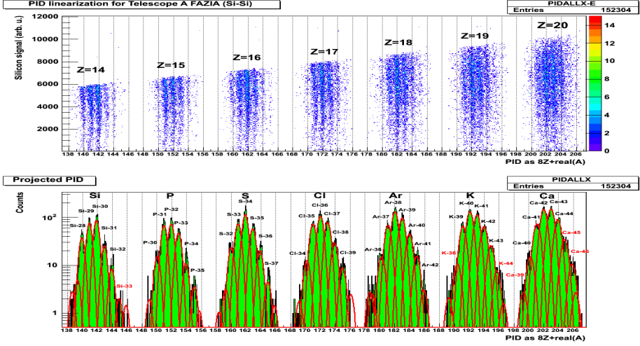
Figure 6: Linearization and isotopic identification in a \Delta E - E silicon telescope.
