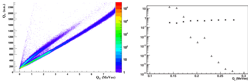
Figure 2: Left: traditional two-dimensional plot Q_s vs Q_t (calibrated into MeVee) illustrating the separation of neutrons (upper branch) and \gamma -rays (lower branch) from an AmBe source; the energetic muons are localized in the latter branch, but at higher total charges Q_t . Right: figure of merit (stars) and neutron area contamination (in %) by \gamma -events (triangles) at one tenth of the neutron maximum.
