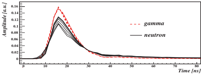
Figure 1: Average signals induced in a BC501A cell by neutrons and \gamma -rays.
