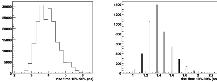
Figure 5: Comparison of the timing properties of a large area pcCVD detector (left panel) and a strip of small area (right panel). See text for more detail.
