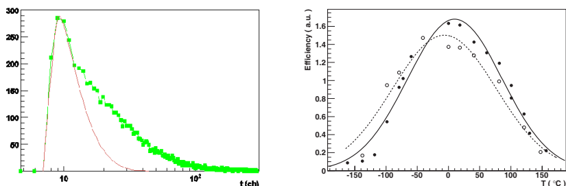
Figure 4: Left: light output induced by \approx 8 AMeV ^{36}\text{Cl} in a 2000 ppm Tl doped CsI(Tl) crystal (symbols connected by a thin line) vs time (4 ns/channel); the other curve stresses the fast peak due to the high Tl doping. Right: data from ref. [12]; the optimum efficiency temperature is lower for \alpha particles (open circles and dashed curve) than for protons (full circles and solid curve).
