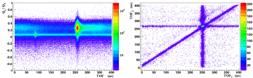
Figure 3: Left: ratio Q_s/Q_t as a function of the time of flight. Right: Correlated events in two BC501A cells in terms of time of flight. See text for more detail.
