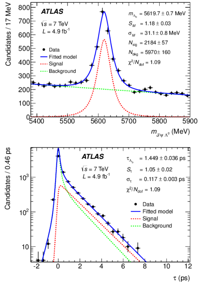
FIG. 3. Projections of the fitted PDF onto the mass (top panel) and the proper decay time (bottom panel) axes for \Lambda_b^0 candidates. The errors of the listed fit result values are statistical only. The \chi^2/N_{\text{dof}} value is calculated from the data set binned in mass and decay time with the number of degrees of freedom, N_{\text{dof}} = 61 .
