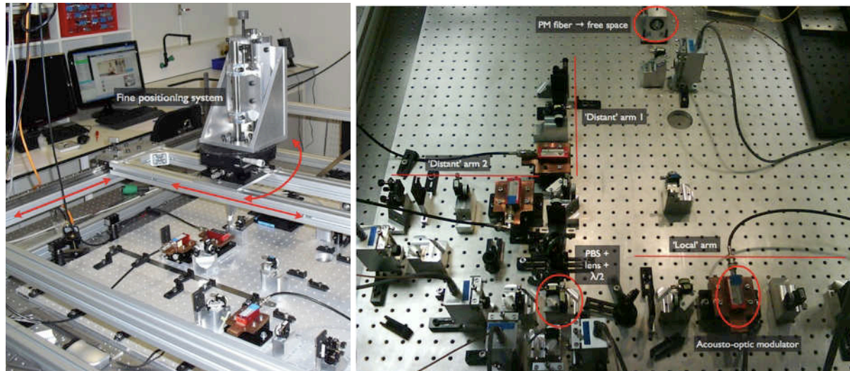
Fig 5. Positioning of the optics components on the aluminium breadboard. Fig 6. The first module mounted on the breadboard.
