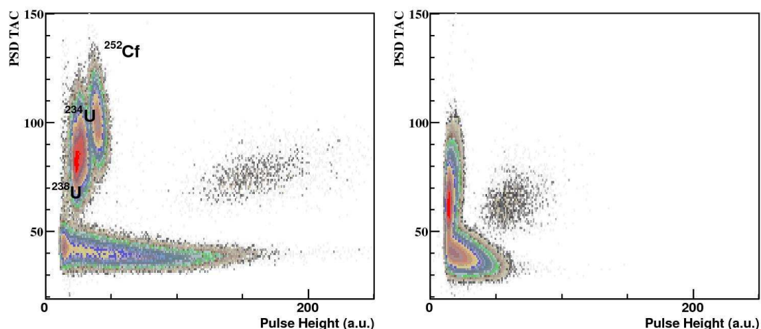
Figure 20: (Color online) Left: (PSD TAC)%PH histogram for a natural uranium concentration of 10 µg/cm 3 . Three \alpha -peaks can be distinguished which corresponds from lower to higher energies to the 238U, 234U and 252Cf decays. Right: same for a concentration of 10 mg/cm 3 . The three \alpha -peaks can not be resolved anymore due to resolution degradation associated to light quenching.
