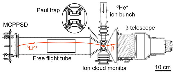
FIG. 1: Top view of the experimental setup. The insert shows the structure of the six stainless steel rings of the Paul trap. See text for details.
