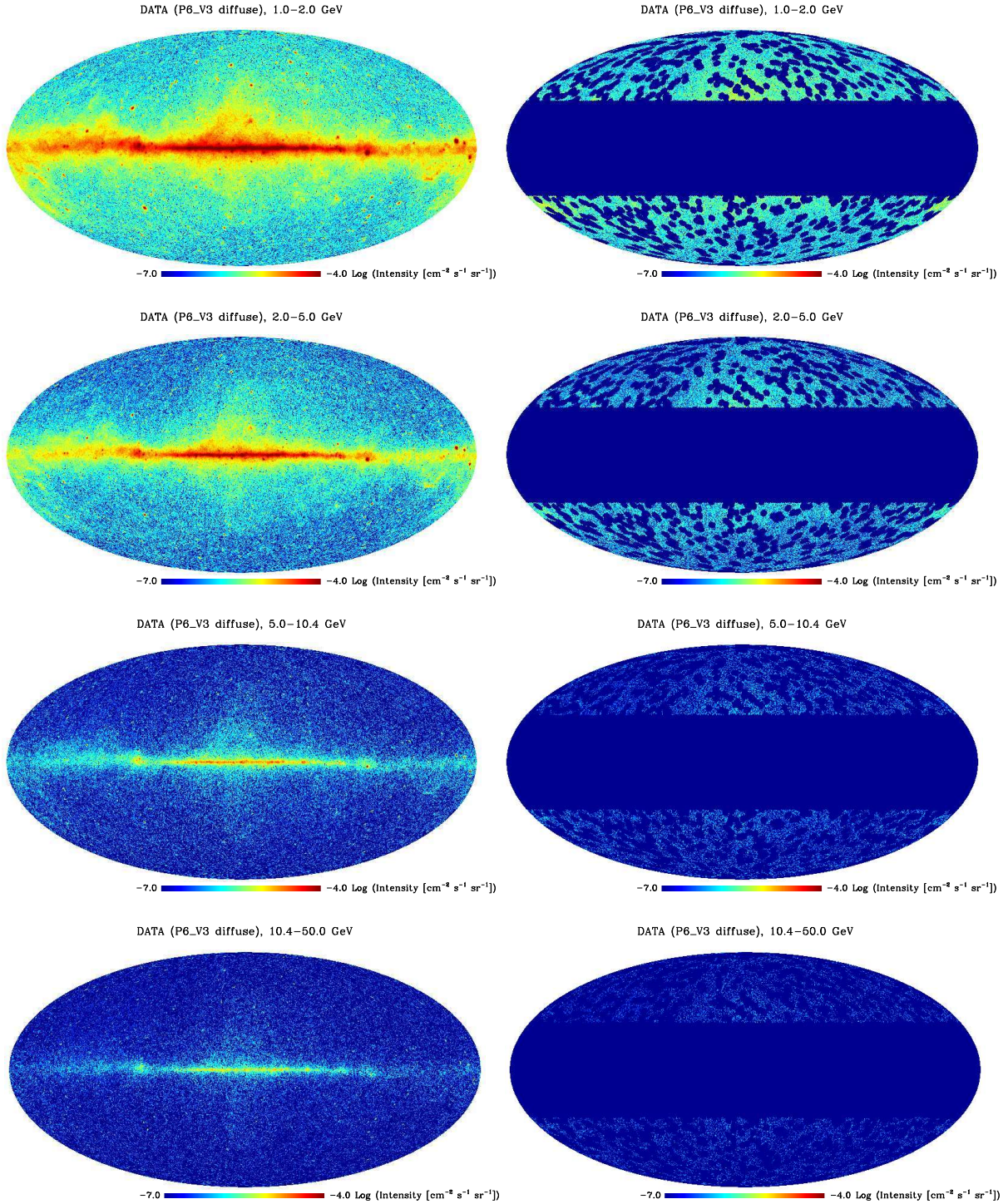
FIG. 1: All-sky intensity maps of the data in the four energy bins used in this analysis, in Galactic coordinates; the map projection is Mollweide. The data shown are the average of the maps of the front- and back-converting events, and are shown unmasked ( left panels ) and with the default mask applied ( right panels ). The mask excludes Galactic latitudes |b| < 30^\circ and a 2^\circ angular radius around each source in the 1FGL catalog. The map images shown have been downgraded in resolution to N_{\text{side}} = 128 to improve the visual quality of the images; however, the analysis was performed on the higher resolution maps as described in the text.
