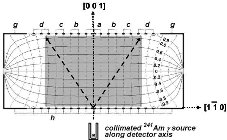
Fig. 1. Detector crystal in cross-section along the (1\bar{1}0) plane, showing the connection scheme of the electrodes and the different charge measurement channels (see text). The equipotentials (full lines) and the field lines (dotted lines) are drawn for detector bias V_p = +1 V. The field is approximately uniform within the core of the device (shaded area). The trajectories of the electrons in the \langle 111 \rangle valleys are drawn schematically (dashed arrowed lines) for an energy deposit at the center of the bottom surface of the crystal, in the hypothetical case that intervalley scattering could be neglected altogether. Electrons would then be collected by the d set of electrodes only.
