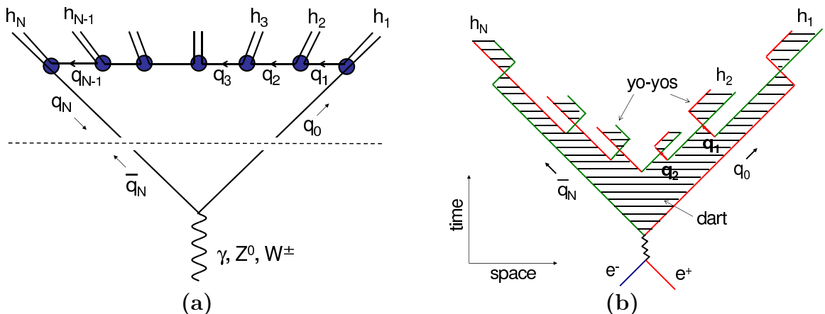
Figure 1: (a) e^+e^- annihilation or W^\pm decay in quark-antiquark \rightarrow hadrons. (b) String fragmentation.
