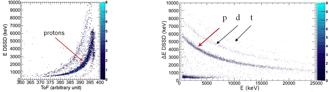
Figure 2: Proton identification in MUST2 telescopes. Left: Energy versus Time of Flight (ToF) selection, where ToF is measured with respect to CATS detector; data of 2 telescopes are summed. Right: \Delta E -E selection, where \Delta E is the energy loss of particles in the first layer of MUST2 detectors, and E the energy deposit of particles in the Si(Li) detector; data of 3 telescopes are summed.
