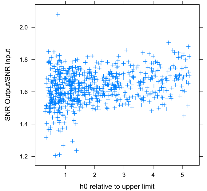
FIG. 9 (color online). Relative increase in SNR of injected test signals from semicoherent to loosely coherent stage. The plot is restricted to injections that passed the coincidence test. The injected strain divided by the upper limit in this band (before injection) is shown on the x axis. The ratio of loosely coherent SNR to semicoherent SNR is shown on the y axis.
