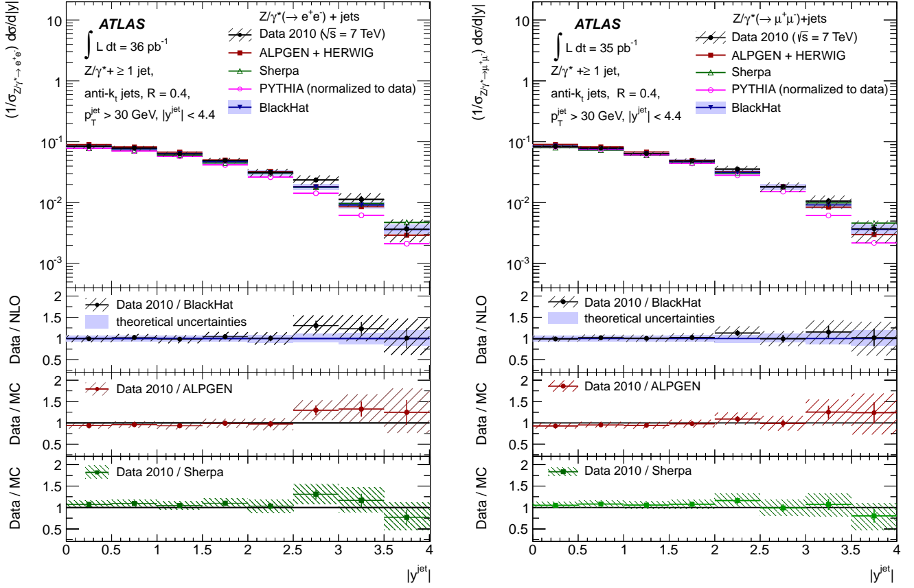
FIG. 8: Measured normalized inclusive jet cross section (1/\sigma_{Z/\gamma^* \rightarrow \ell^+ \ell^-}) d\sigma/d|y| (black dots) in (left) Z/\gamma^* (\rightarrow e^+ e^-) + \text{jets} and (right) Z/\gamma^* (\rightarrow \mu^+ \mu^-) + \text{jets} production as a function of |y| , in events with at least one jet with p_T > 30 GeV and |y| < 4.4 in the final state, and normalized by \sigma_{Z/\gamma^* \rightarrow e^+ e^-} and \sigma_{Z/\gamma^* \rightarrow \mu^+ \mu^-} Drell-Yan cross sections, respectively.
