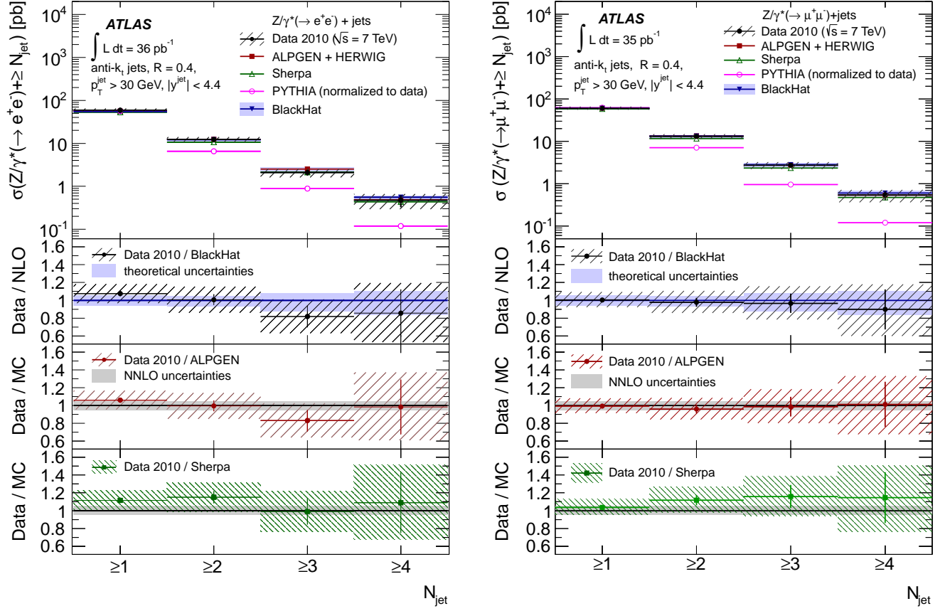
FIG. 3: Measured cross section \sigma_{N_{\text{jet}}} (black dots) for (left) Z/\gamma^*(\rightarrow e^+e^-)+\text{jets} and (right) Z/\gamma^*(\rightarrow \mu^+\mu^-)+\text{jets} production as a function of the inclusive jet multiplicity, for events with at least one jet with p_T > 30 GeV and |y| < 4.4 in the final state. In this and subsequent figures 4 - 14 the error bars indicate the statistical uncertainty and the dashed areas the statistical and systematic uncertainties added in quadrature. The measurements are compared to NLO pQCD predictions from BlackHat, as well as the predictions from ALPGEN and Sherpa (both normalized to the FEWZ value for the total cross section), and PYTHIA (normalized to the data as discussed in Section XII).
