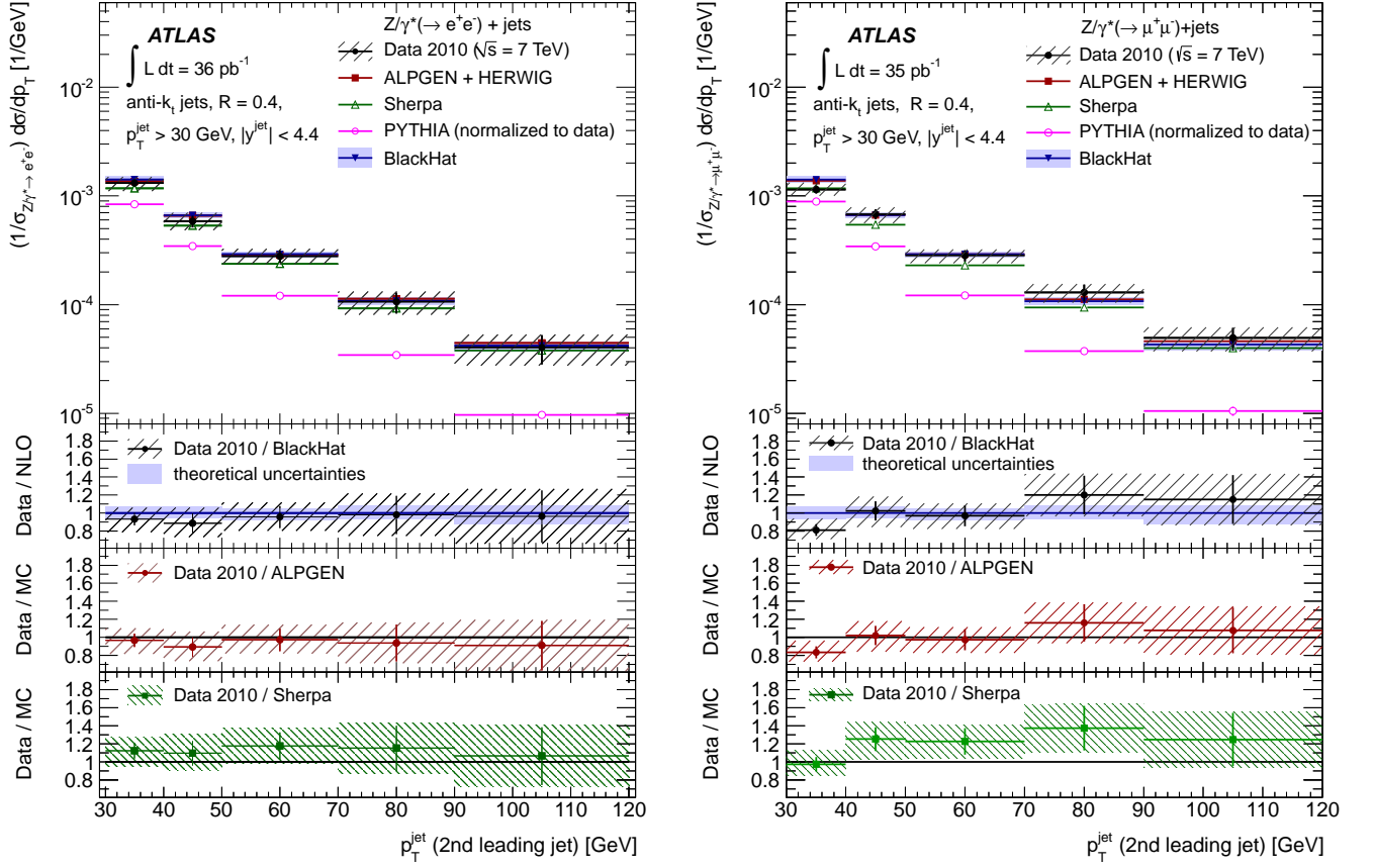
FIG. 7: Measured normalized jet cross section (1/\sigma_{Z/\gamma^* \rightarrow \ell^+ \ell^-}) d\sigma/dp_T (black dots) in (left) Z/\gamma^* (\rightarrow e^+ e^-) + \text{jets} and (right) Z/\gamma^* (\rightarrow \mu^+ \mu^-) + \text{jets} production as a function of the second-leading jet p_T , in events with at least two jets with p_T > 30 GeV and |y| < 4.4 in the final state, and normalized by \sigma_{Z/\gamma^* \rightarrow e^+ e^-} and \sigma_{Z/\gamma^* \rightarrow \mu^+ \mu^-} Drell-Yan cross sections, respectively.
