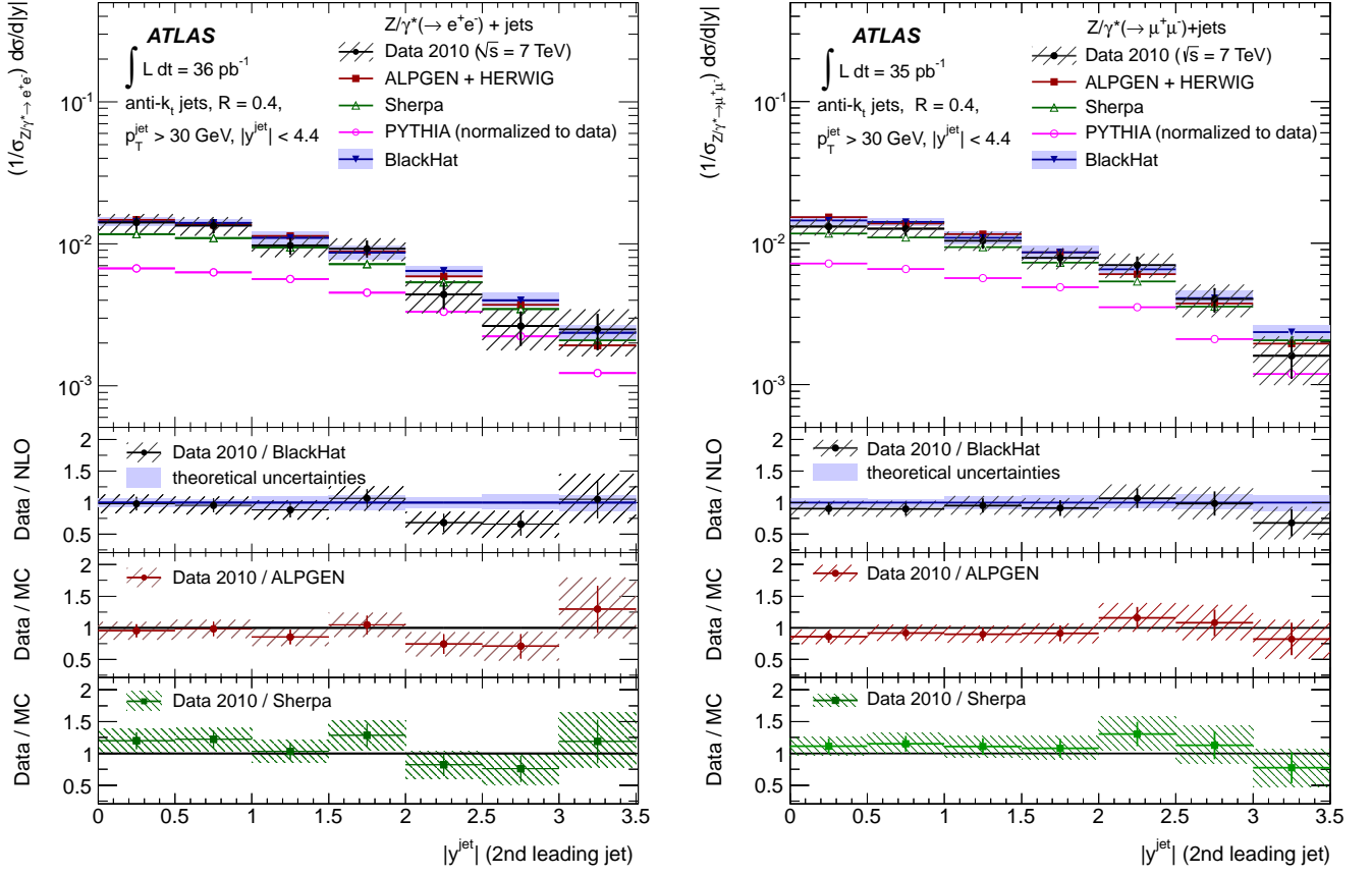
FIG. 10: Measured normalized jet cross section (1/\sigma_{Z/\gamma^* \rightarrow \ell^+ \ell^-}) d\sigma/d|y| (black dots) in (left) Z/\gamma^*(\rightarrow e^+ e^-) + \text{jets} and (right) Z/\gamma^*(\rightarrow \mu^+ \mu^-) + \text{jets} production as a function of the second-leading jet |y| , in events with at least two jets with p_T > 30 GeV and |y| < 4.4 in the final state, and normalized by \sigma_{Z/\gamma^* \rightarrow e^+ e^-} and \sigma_{Z/\gamma^* \rightarrow \mu^+ \mu^-} Drell-Yan cross sections, respectively.
