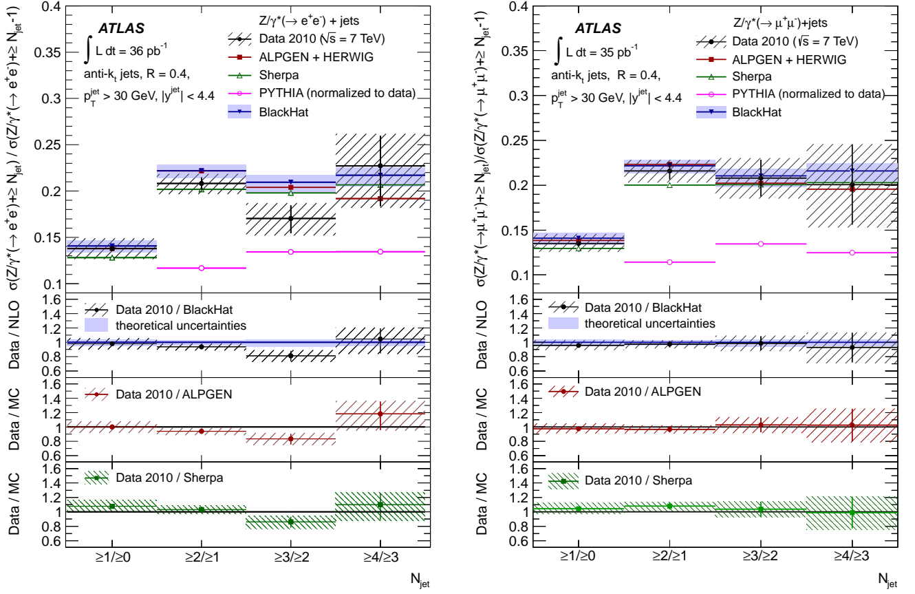
FIG. 4: Measured ratio of cross sections ( \sigma_{N_{\text{jet}}}/\sigma_{N_{\text{jet}}-1} ) (black dots) for (left) Z/\gamma^*(\rightarrow e^+e^-)+\text{jets} and (right) Z/\gamma^*(\rightarrow \mu^+\mu^-)+\text{jets} production as a function of the inclusive jet multiplicity, for events with at least one jet with p_T > 30 GeV and |y| < 4.4 in the final state.
