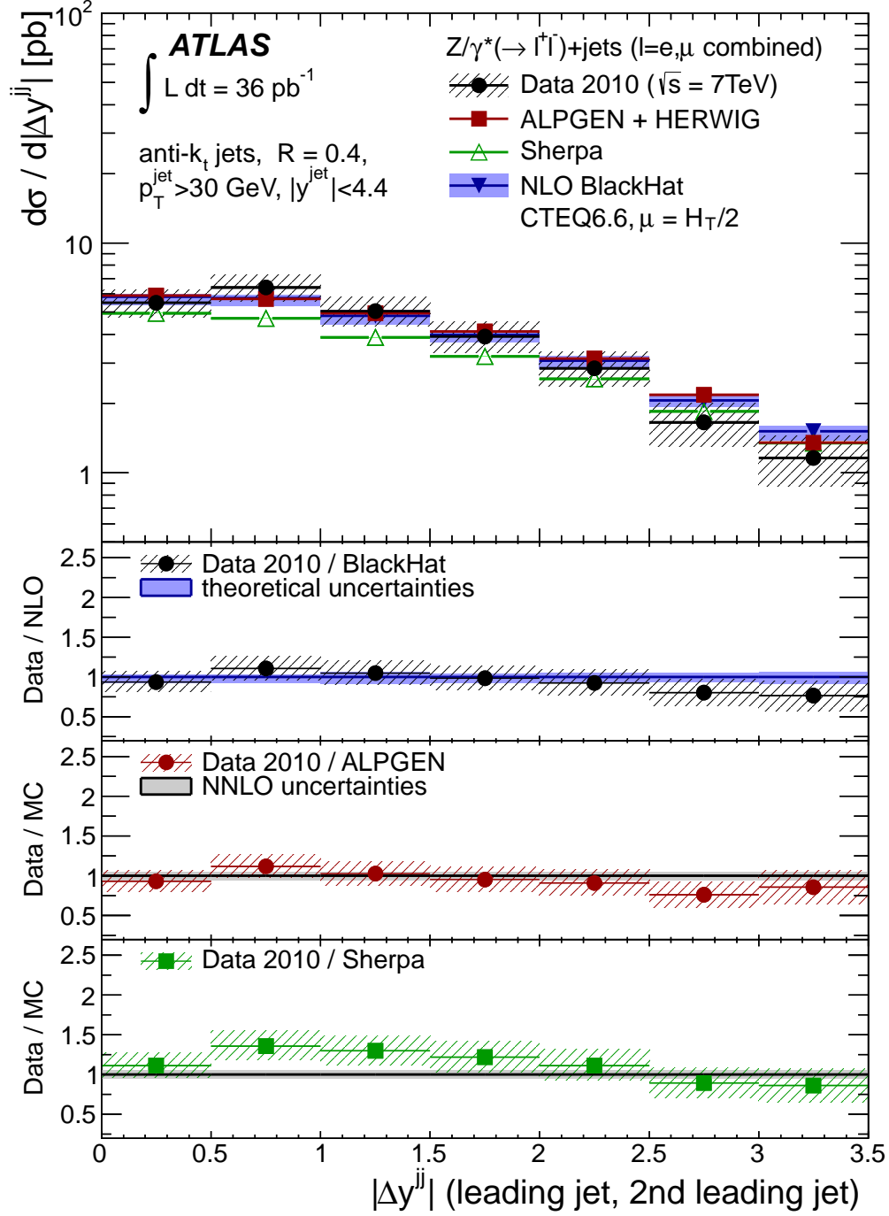
FIG. 24: Measured dijet cross section d\sigma/d|\Delta y^{jj}| (black dots) in Z/\gamma^*(\rightarrow \ell^+\ell^-)+\text{jets} production as a function of the rapidity separation of the two leading jets |\Delta y^{jj}| , in events with at least two jets with p_T > 30 \text{ GeV} and |y| < 4.4 in the final state.
