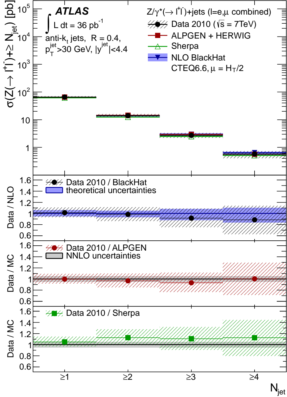
FIG. 15: Measured cross section \sigma_{N_{\text{jet}}} (black dots) in Z/\gamma^*(\rightarrow \ell^+\ell^-)+\text{jets} production as a function of the inclusive jet multiplicity, for events with at least one jet with p_T > 30 \text{ GeV} and |y| < 4.4 in the final state. In this and subsequent figures 16 - 26 the error bands indicate the total uncertainty from the combination of electron and muon results. The measurements are compared to NLO pQCD predictions from BlackHat, as well as the predictions from ALPGEN and Sherpa (both normalized to the FEWZ value for the total cross section).
