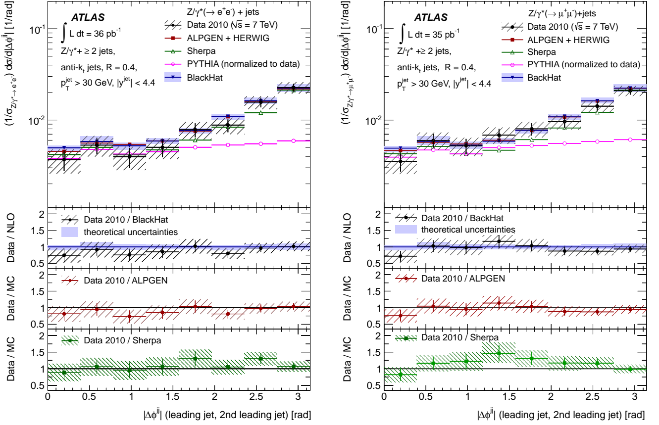
FIG. 13: Measured normalized dijet cross section (1/\sigma_{Z/\gamma^* \rightarrow \ell^+ \ell^-}) d\sigma/d|\Delta\phi^{jj}| (black dots) in (left) Z/\gamma^*(\rightarrow e^+e^-)+ jets and (right) Z/\gamma^*(\rightarrow \mu^+\mu^-)+ jets production as a function of the azimuthal separation of the two leading jets |\Delta\phi^{jj}| , in events with at least two jets with p_T > 30 GeV and |y| < 4.4 in the final state, and normalized by \sigma_{Z/\gamma^* \rightarrow e^+e^-} and \sigma_{Z/\gamma^* \rightarrow \mu^+\mu^-} Drell-Yan cross sections, respectively.
