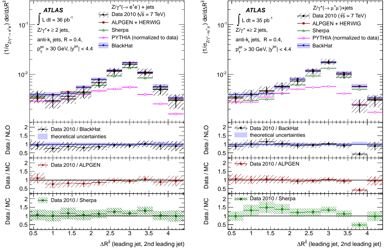
FIG. 14: Measured normalized dijet cross section (1/\sigma_{Z/\gamma^* \rightarrow \ell^+\ell^-})d\sigma/d\Delta R^{jj} (black dots) in (left) Z/\gamma^* \rightarrow e^+e^- + \text{jets} and (right) Z/\gamma^* \rightarrow \mu^+\mu^- + \text{jets} production as a function of the angular separation ( y - \phi space) of the two leading jets \Delta R^{jj} , in events with at least two jets with p_T > 30 \text{ GeV} and |y| < 4.4 in the final state, and normalized by \sigma_{Z/\gamma^* \rightarrow e^+e^-} and \sigma_{Z/\gamma^* \rightarrow \mu^+\mu^-} Drell-Yan cross sections, respectively.
