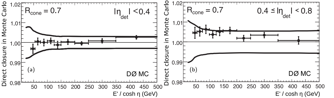
FIG. 22: Closure test of jet energy scale in MC for (a) |\eta_{det}| < 0.4 and (b) 0.4 < |\eta_{det}| < 0.8 . The band outlined by the solid curves corresponds to the uncertainties in the extraction of jet energy scale in MC which are mainly statistical.
