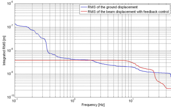
Figure 7: Integrated RMS obtained with feedback control
