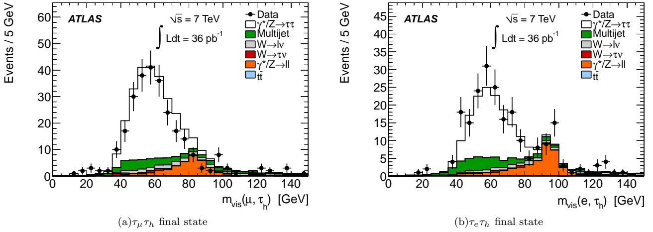
FIG. 3. The distributions of the visible mass of the combination of the \tau candidate and the lepton are shown for the (a) \tau\mu\tau_h and (b) \tau_e\tau_h final states. These distributions are shown after the full event selection, except for the visible mass window requirement.
