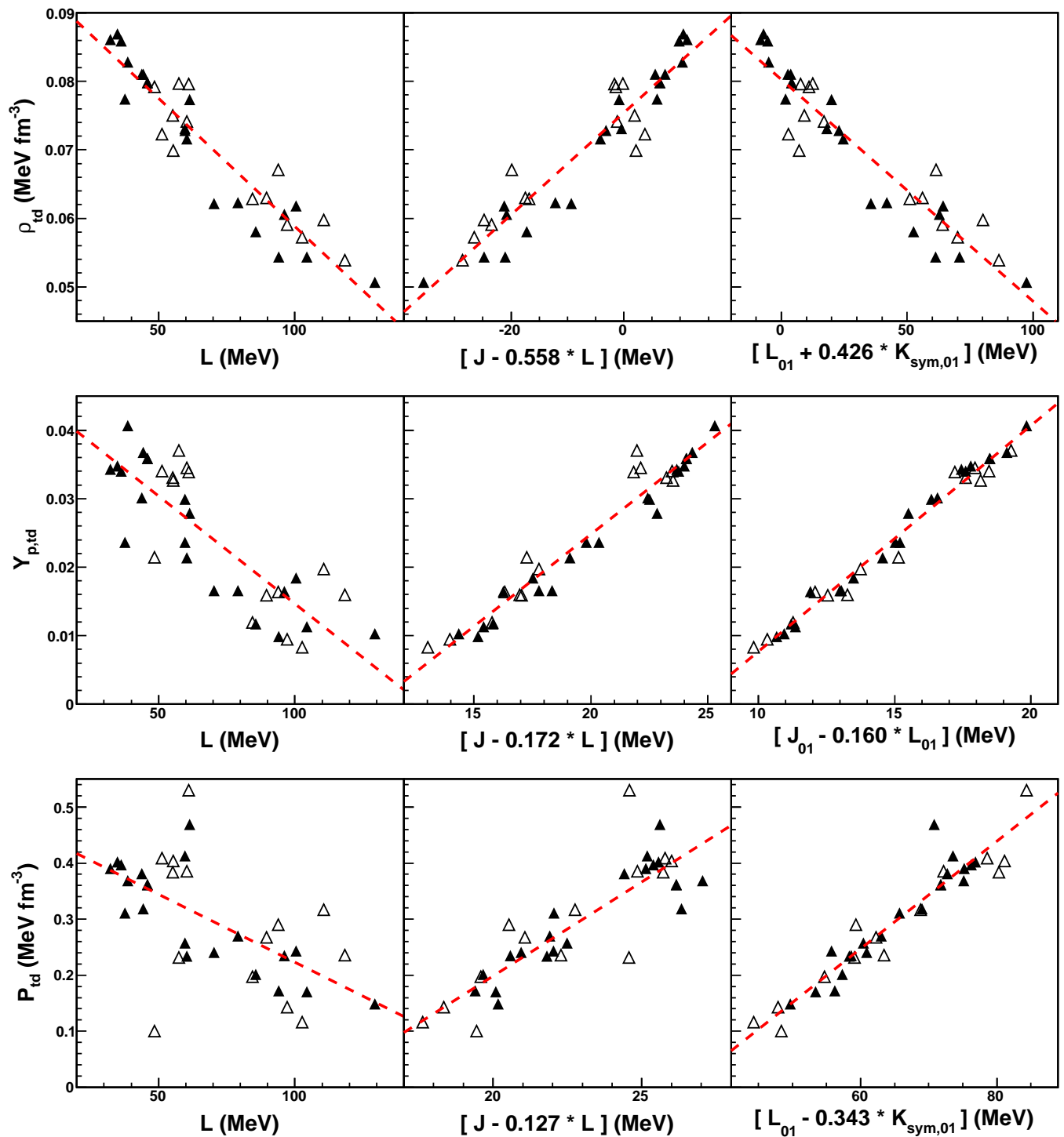
FIG. 17: Correlations between the dynamic core-crust transition properties and GLDM coefficients (see text).
