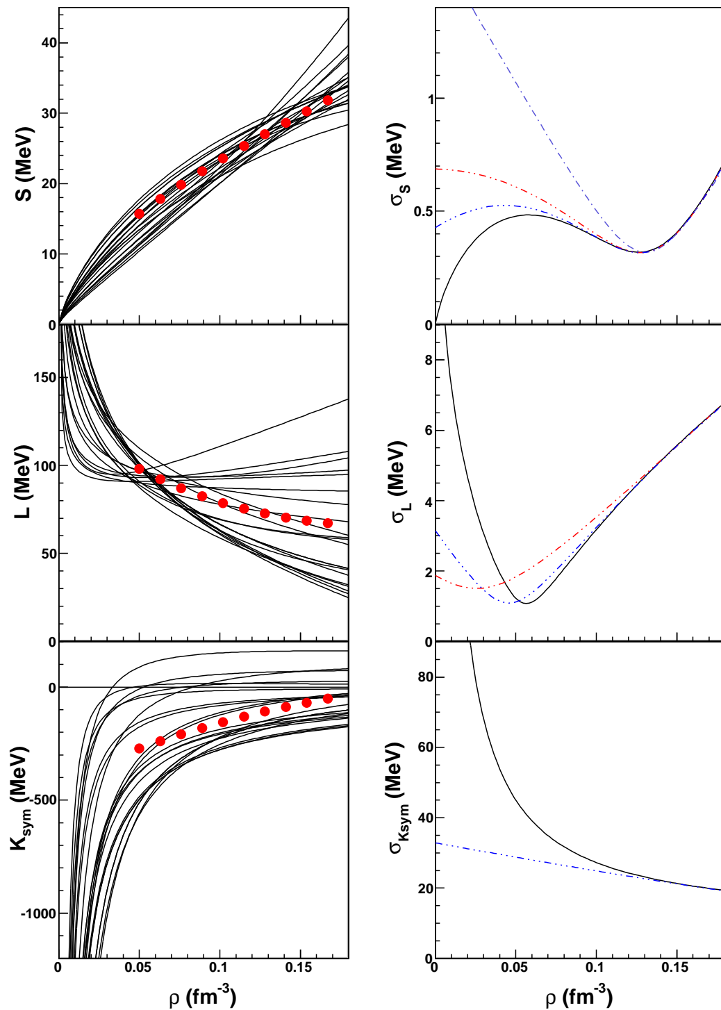
FIG. 2: (Color online) Skyrme models: Left: symmetry energy value (top), slope (center) and curvature (bottom) as a function of the density, calculated with complete functionals. BHF results are indicated for comparison (dots). Right: the corresponding variance for a calculation using the complete functionals (full line) and the GLDM up to different orders: D_1(\rho_0) (dot-dashed line), D_2(\rho_0) (2dot-dashed line) and D_3(\rho_0) (3dot-dashed line).
