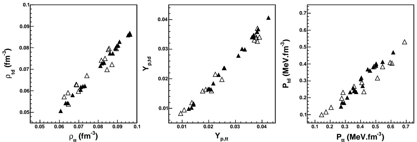
FIG. 16: (Color online) Comparison between the transition taken at dynamic (td) and thermodynamic (tt) spinodal for different Skyrme (full symbols) and relativistic (empty symbols) models: density (left), proton fraction (center) and pressure (right).
