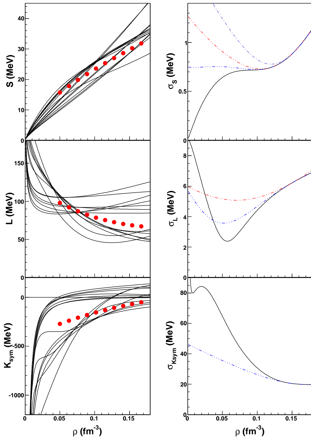
FIG. 3: (Color online) Relativistic models: Left: symmetry energy value (top), slope (center) and curvature (bottom) as a function of the density, calculated with complete functionals. BHF results are indicated for comparison (dots). Right: the corresponding variance for a calculation using the complete functionals (full line) and the GLDM up to different orders: D_1(\rho_0) (dot-dashed line), D_2(\rho_0) (2dot-dashed line) and D_3(\rho_0) (3dot-dashed line).
