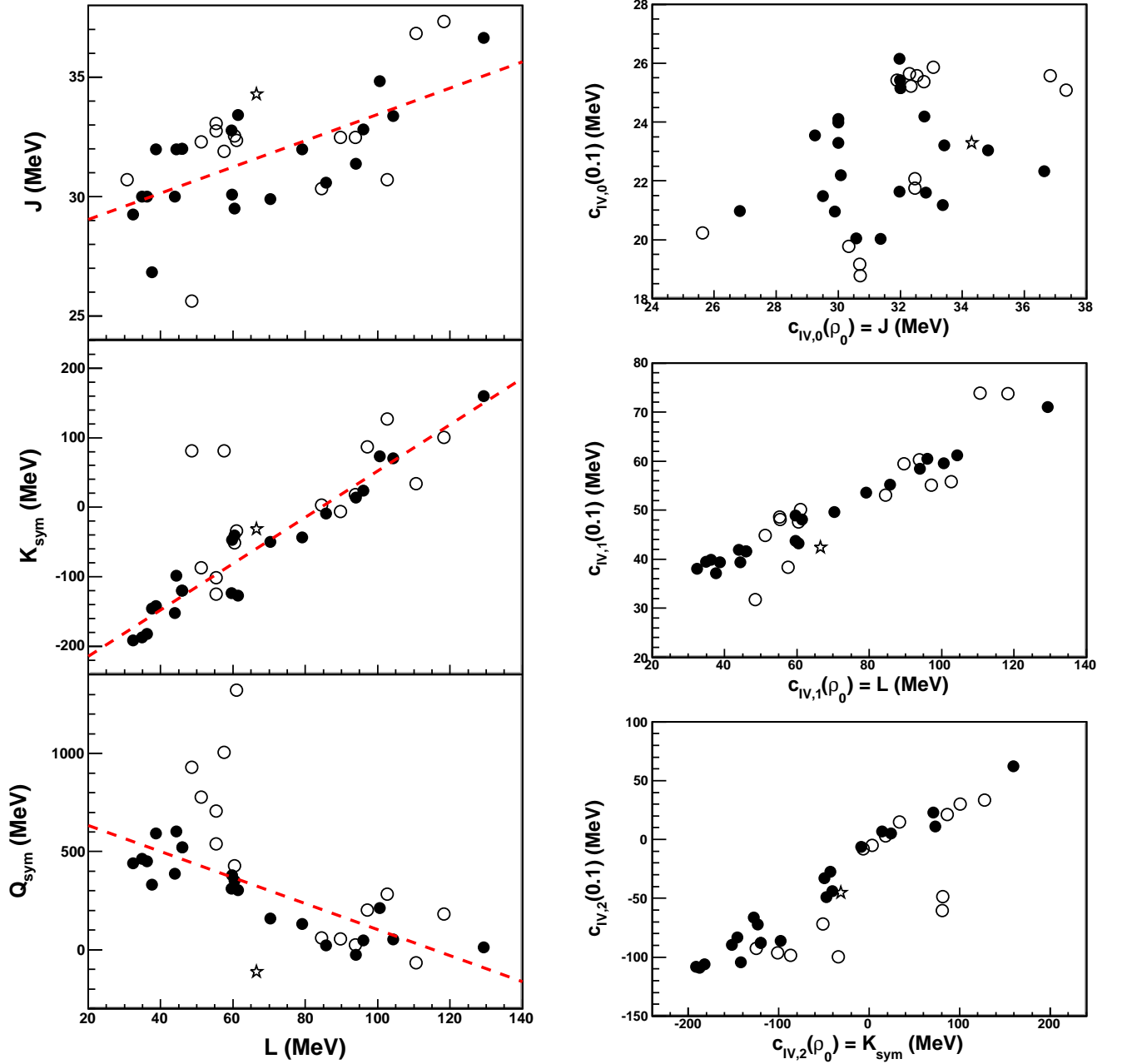
FIG. 1: (Color online) Correlations between different GLDM coefficients c_{IV,n} . Left : at saturation density, relation between L and other coefficients c_{IV,n}(\rho_0) , namely J (top), K_{\text{sym}} (center) and Q_{\text{sym}} (bottom). Right : relation between coefficients c_{IV,n} defined at reference density \rho_0 or \rho=0.1 \text{ fm}^{-3} . Results are shown for different Skyrme models (full symbols), relativistic models (empty symbols), and BHF (star). BHF-1 is used at saturation density, and BHF-2 is used at \rho=0.1 \text{ fm}^{-3} .
