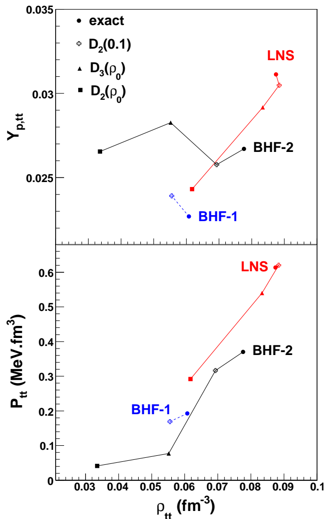
FIG. 5: (Color online) Comparison between exact and GLDM versions of three functionals based on BHF calculations: LNS (Skyrme-type force including constraints from BHF), BHF-1 (fit of the BHF EOS including densities in the range \rho = [0.1; 0.35] \text{fm}^{-3} ), and BHF-2 (fit of the BHF EOS including lower densities, in the range \rho = [0.05; 0.18] \text{fm}^{-3} ).
