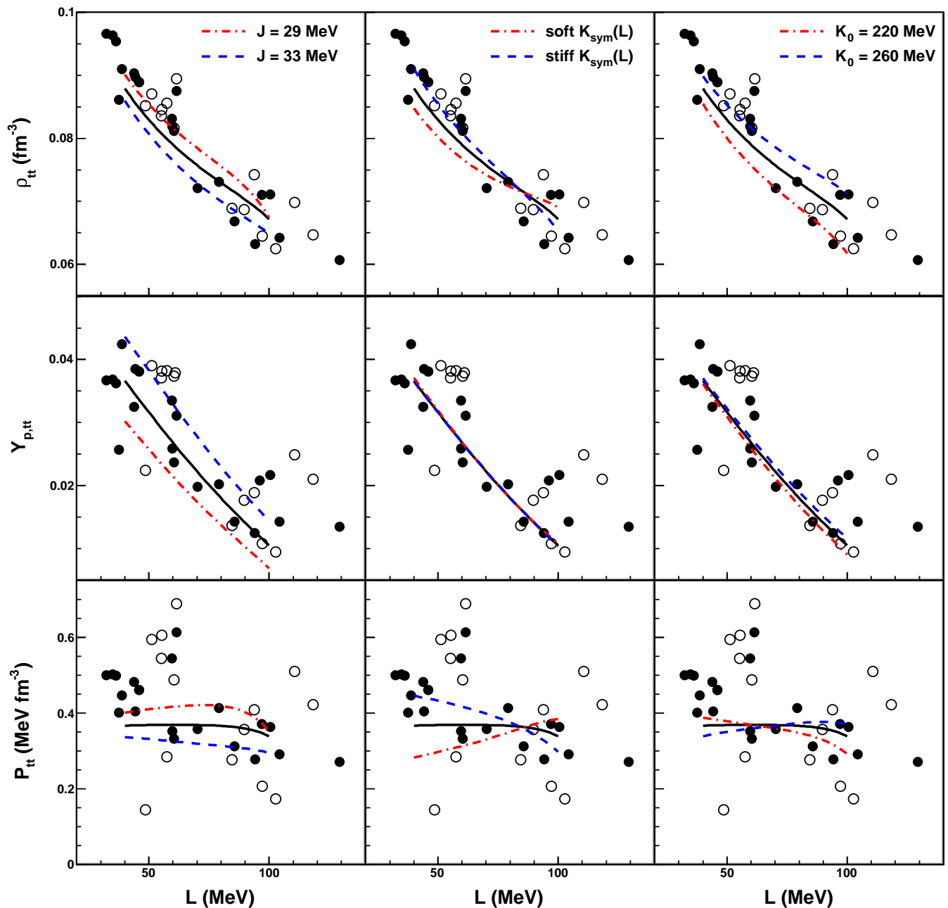
FIG. 12: (Color online) Predictions of the standard schematic model for the transition density, proton fraction and pressure, compared with complete effective models: Skyrme (full symbols) and relativistic (empty symbols) models. Left: varying the symmetry energy at saturation, J . Center: varying the relation K_{\text{sym}}(L) . Right: varying the incompressibility at saturation K_0 .
