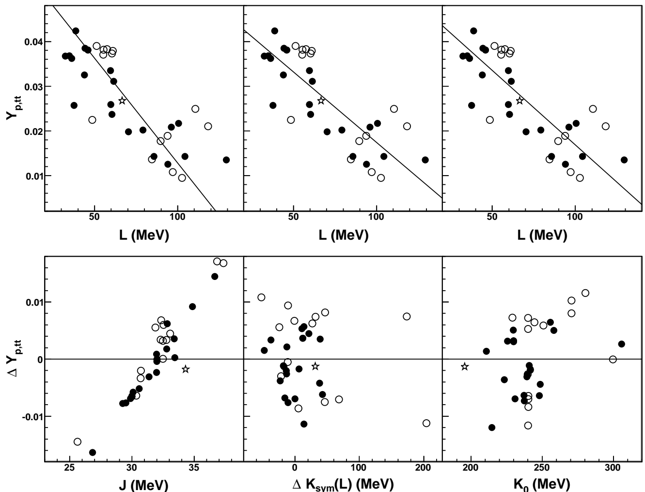
FIG. 13: Relation between the dispersion of Y_{p,tt}(L) and the dispersion of GLDM properties ( J , K_0 , \Delta K_{\text{sym}}(L) ) associated with the different models (see text). Nuclear models: Skyrme (full symbols), relativistic (empty symbols), and BHF-2 (star).
