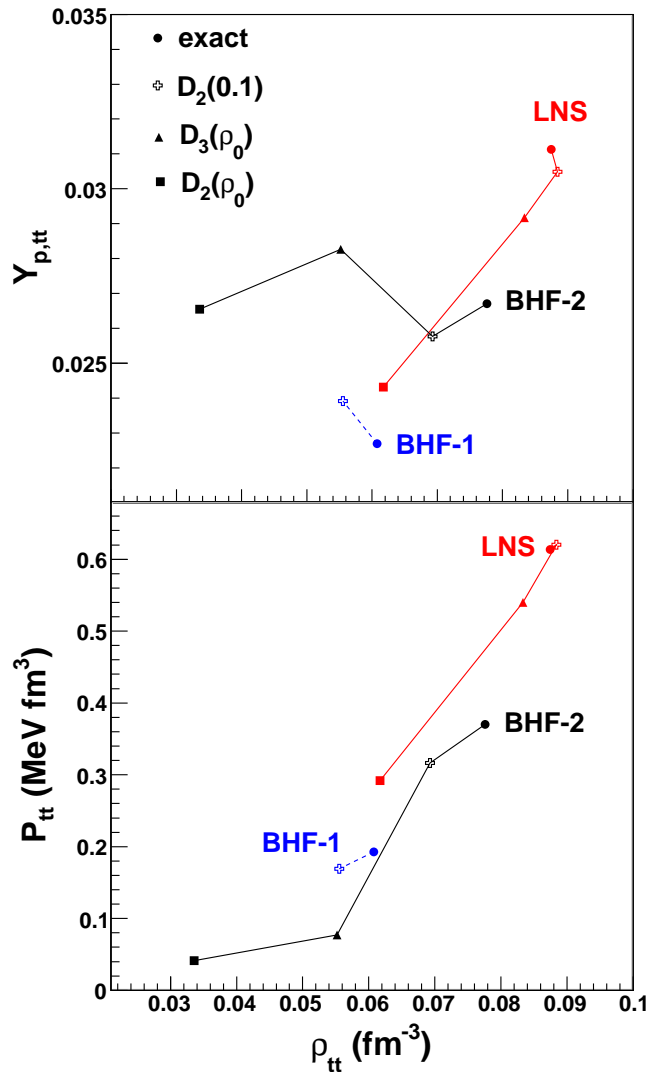
FIG. 5: (Color online) Comparison between exact and GLDM versions of three functionals based on BHF calculations: LNS [47] (Skyrme-type force including constraints from BHF), BHF-1 (fit of the BHF EOS including densities in the range \rho = [0.1; 0.35] \text{fm}^{-3} ), and BHF-2 (fit of the BHF EOS including lower densities, in the range \rho = [0.05; 0.18] \text{fm}^{-3} ).
