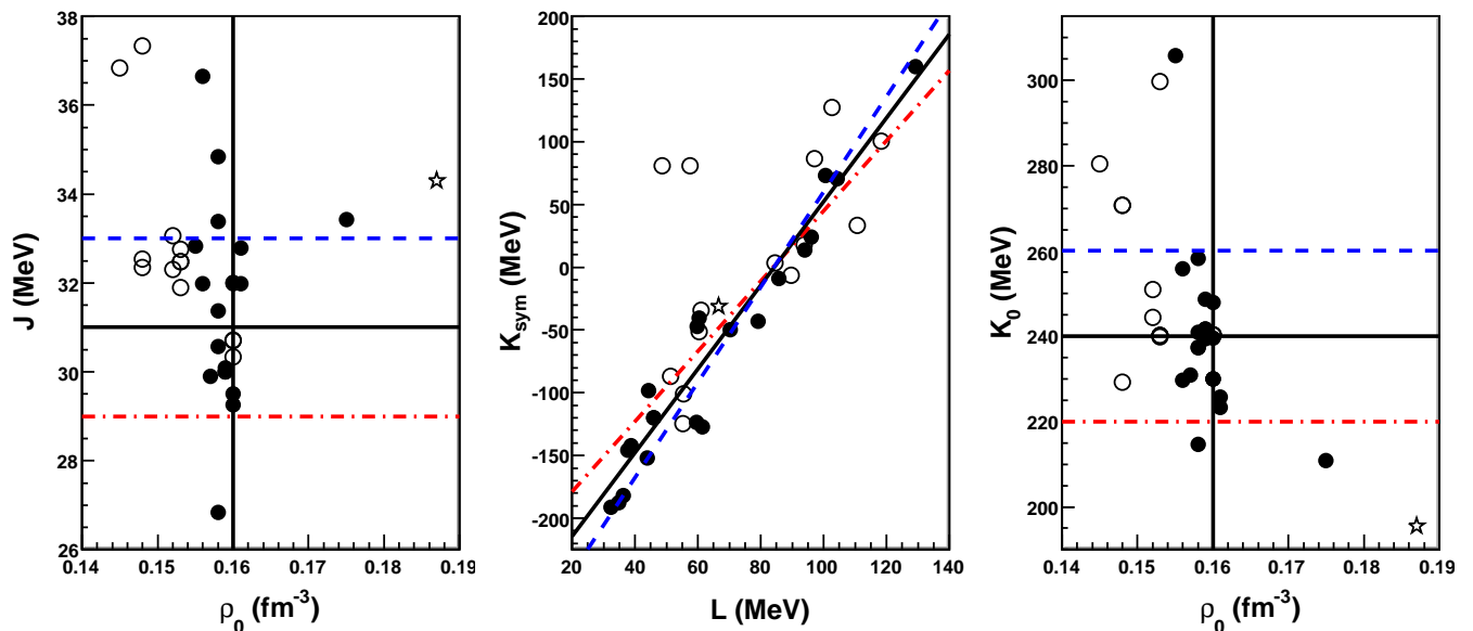
FIG. 11: (Color online) Typical variation for the values of J , K_{\text{sym}}(L) and K_0 . We represent these quantities for different Skyrme models (full symbols), relativistic models (empty symbols), and BHF-1 (star). The lines show the different values which are used for the standard schematic model (see text).
