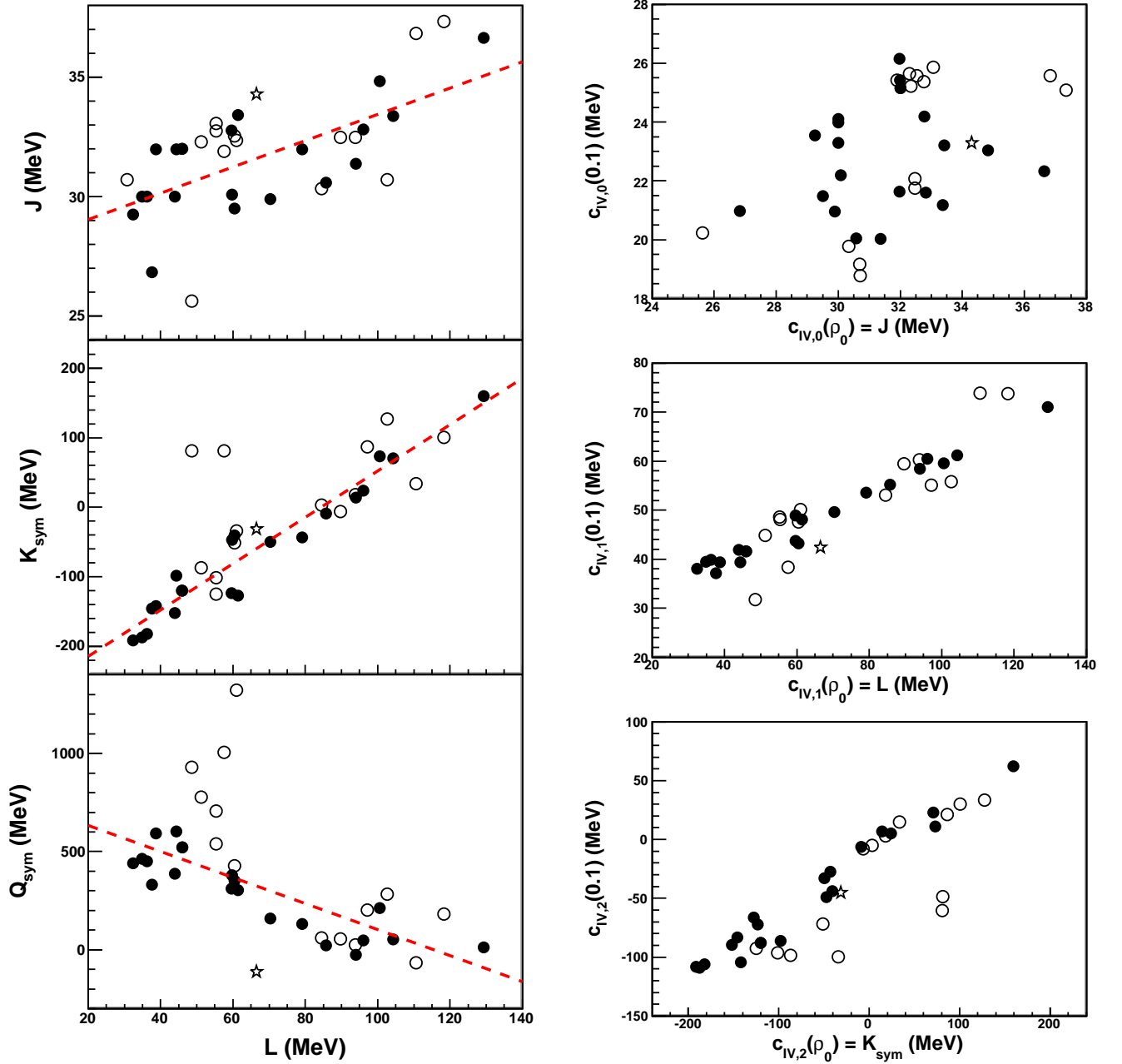
FIG. 1: (Color online) Correlations between different GLDM coefficients c_{IV,n} . Left : at saturation density, relation between L and other coefficients c_{IV,n}(\rho_0) , namely, J (top), K_{\text{sym}} (center) and Q_{\text{sym}} (bottom). Right : relation between coefficients c_{IV,n} defined at reference density \rho_0 or \rho=0.1 \text{ fm}^{-3} . Results are shown for different Skyrme models (full symbols), relativistic models (empty symbols), and BHF (star). BHF-1 is used at saturation density, and BHF-2 is used at \rho=0.1 \text{ fm}^{-3} .
