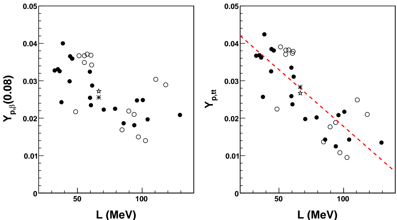
FIG. 6: (Color online) Effect of L on the proton fraction at \beta equilibrium for a fixed density \rho=0.08 \text{ fm}^{-3} (left) and at thermodynamic spinodal crossing (right), for different nuclear models: Skyrme (full symbols), relativistic (empty symbols), BHF-2 (star) and BHF-2 para (asterisk).
