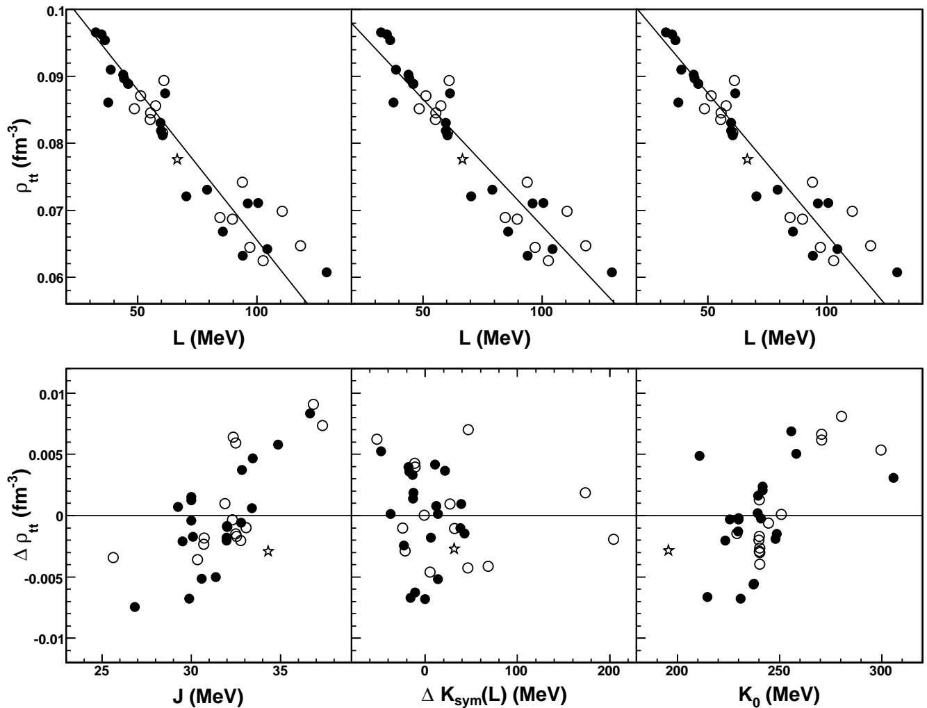
FIG. 14: Relation between the dispersion of \rho_{tt}(L) and the dispersion of GLDM properties ( J , K_0 , \Delta K_{\text{sym}}(L) ) associated with the different models (see text). Nuclear models: Skyrme (full symbols), relativistic (empty symbols), and BHF-2 (star).
