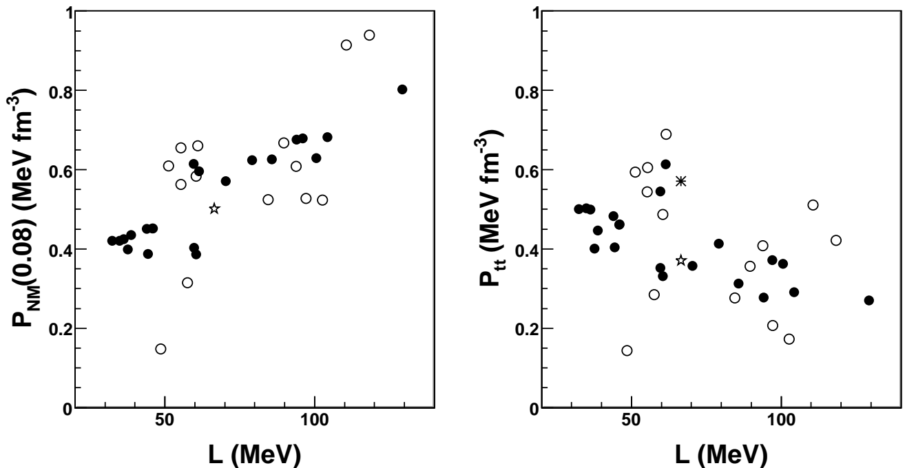
FIG. 9: (Color online) Impact of L on the pressure of neutron-rich matter at sub-saturation density, for different nuclear models: Skyrme (full symbols), relativistic (empty symbols), BHF-2 (star) and BHF-2 para (asterisk). Both BHF-2 results are identical for neutron matter. Left: pressure of pure neutron matter, for a fixed density typical of the transition: \rho=0.08 \text{ fm}^{-3} . Right: thermodynamic transition pressure.
