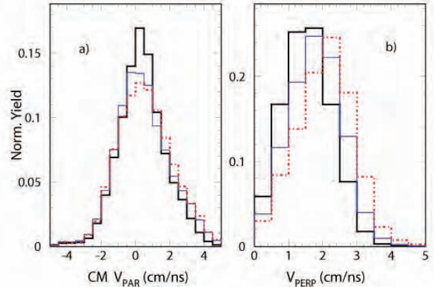
Fig. 1: a) Parallel velocity distributions for events with 3 IMFs sorted as a function of fragment charge. Black thick line (biggest charge), thin blue line (intermediate), red dot-dashed (smallest charge); b) the same for the IMFs transverse velocity.
