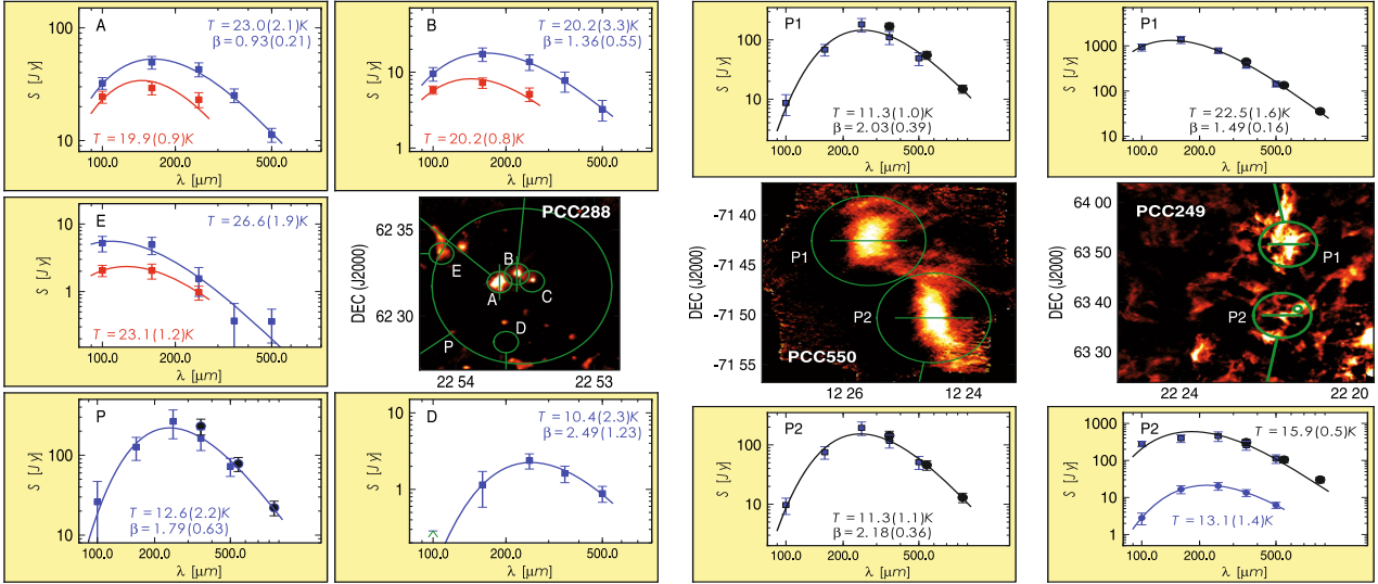
Fig. 1. Spectral energy distributions of selected areas in PCC288 ( left ), PCC550 ( middle ), and PCC249 ( right ). The maps show the PACS 100 \mu\text{m} (PCC288 and PCC249) or 160 \mu\text{m} (PCC550) intensity. For PCC288, greybody fits are presented for 100–500 \mu\text{m} data using 73'' apertures (blue squares and lines; the smaller circles on the map) and for 110–250 \mu\text{m} data using 36'' apertures (red squares and lines). For PCC288-P (and the areas in PCC550 and PCC249, the fits employ 9' apertures and include the Planck fluxes (black circles). If the value of \beta is not quoted, a fixed value of \beta = 2.0 was assumed. The vertical and horizontal lines indicate the cuts used in Fig. 2. The source coordinates are given in Table 2.
