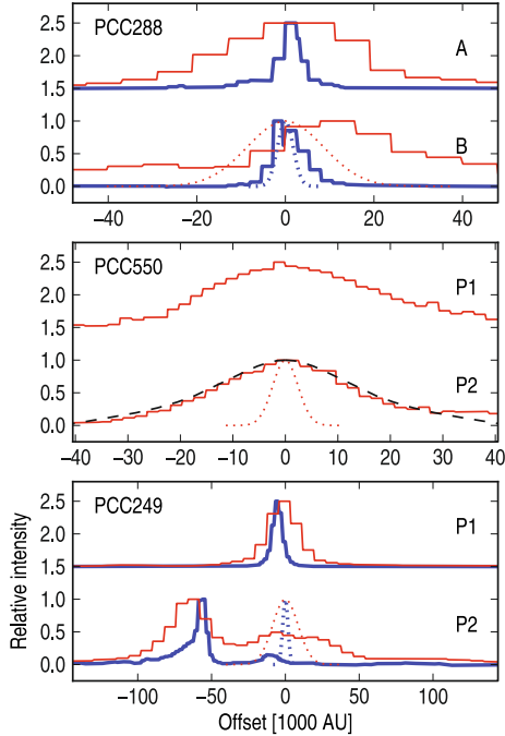
Fig. 2. Intensity profiles at 100\ \mu\text{m} (thick blue lines) and 350\ \mu\text{m} (thin red lines) across selected beam cores along the cuts shown in Fig. 1. The dotted lines indicate beam sizes. Positive offsets correspond to positions west or north of the reference position (see Table 2). For PCC550, the dashed line shows the column density profile of a Bonnor-Ebert sphere (Bonnor 1956; T = 11\ \text{K} , \xi = 6.99 , P_{\text{ext}} = 10^4\ \text{K cm}^{-3} ) without beam convolution. Each curve has been normalized with its peak value.
