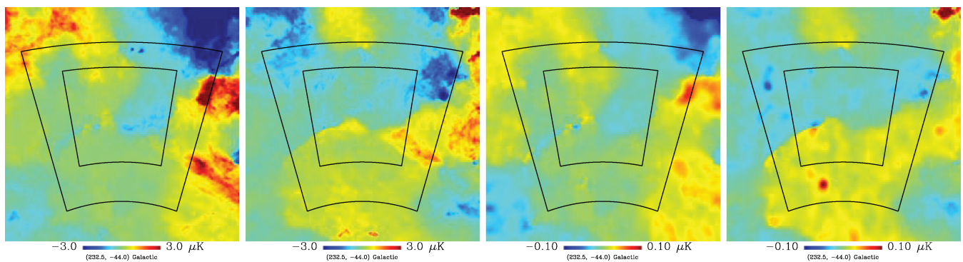
Figure 3. Simulated thermal dust (left) and synchrotron (right) Stokes Q and U templates at 150 GHz, for the ‘basic model’ described in Section 4. The high degree of correlation between the two components on large angular scales is imposed by polarization angle template we assume. The two foregrounds have roughly the same amplitude around 70 GHz.
