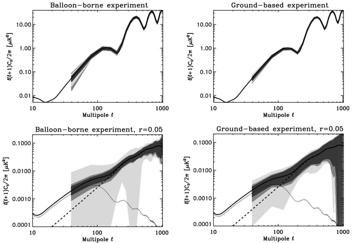
Figure 1. Variance of the estimated E-mode (upper panels) and B-mode power spectrum (lower panels) for the balloon-borne (left panels) and ground-based (right panels) sky-coverage as shown in Fig. 2. From darkest to lightest grey: Fisher estimation (i.e. the so-called f_{\text{sky}} approximation), standard deviation of 500 Monte Carlo simulations using the pure pseudo- C_\ell 's estimator as implemented in XPURE and, standard deviation of 500 Monte Carlo simulations using the standard pseudo- C_\ell 's estimator as implemented in XPOL. We stress that XPURE provides lower variances than XPOL for the B-modes, while XPOL performs better for the E-modes.
