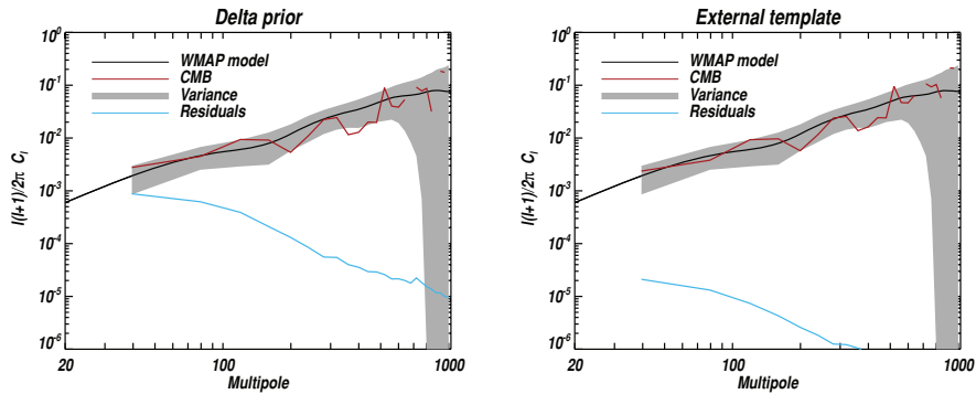
Figure 10. Ground-based experiment. B-mode power spectra of the residuals in the CMB map, as in Fig. 7. Left: The basic case, imposing the dust spectral index value recovered by the balloon-borne experiment (to be compared with the first panel of Fig. 9). Right: Subtracting a synchrotron template with an amplitude known to be within a 10 per cent.
