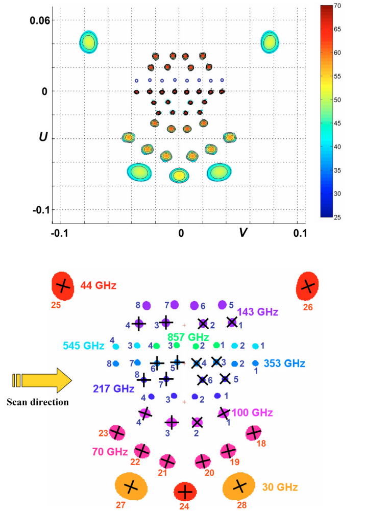
Fig. 4. The footprint of the focal plane as seen by an observer at infinity. The top panel shows predicted contours of each main beam (averaged across the band); the horizontal and vertical axis are in U = \sin(\theta) \times \cos(\phi) and V = \sin(\theta) \times \sin(\phi) (where \theta is the angle around X_{\text{TEL}} and \phi the angle around Y_{\text{TEL}} , offset to the centre of each beam). The colour scale is in dBi. Patterns for the multi-moded horns (545, 857 GHz) are not in final form; only their location relative to the other beams is indicated. The bottom panel is an explanatory guide. Frequencies are identified by colours; the horn identification numbers are also indicated (LFI horns in red, HFI horns in blue). The crossed lines indicate the direction of sensitivity to linear polarisation for pairs of bolometers or radiometers within each horn (horns with no cross correspond to bolometers sensitive to total power only). The plate scale is \sim 32^\circ/\text{m} . The largest extent of the footprint on the sky is almost 9^\circ along the scan direction (i.e., between the outermost 44 GHz beams). The scan direction shown is that of the beams across the sky, i.e., the rightmost horn (e.g., 28) crosses a celestial source before the leftmost (e.g. 27) does. The radius of the circle on the sky described by each horn decreases from bottom to top on this diagram, i.e. horn 27 has a radius of 88^\circ 90' and horn 25 of 82^\circ 59' .
