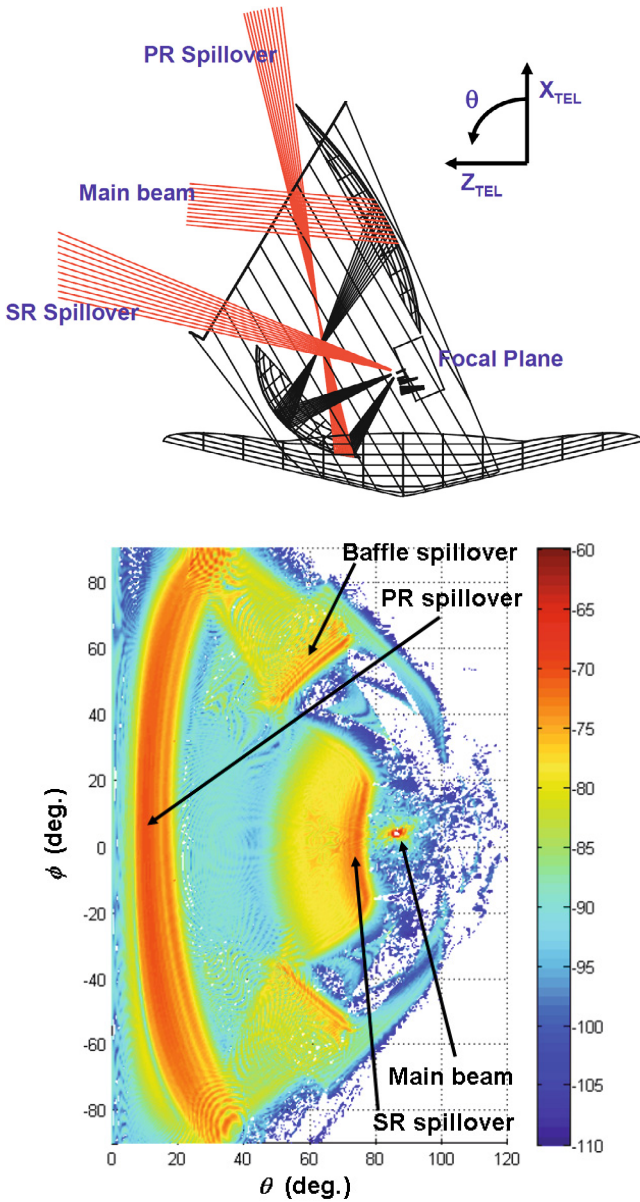
Fig. 5. A typical far side lobe pattern for Planck (in this case at 100 GHz), showing the main features of interest. The horizontal axis corresponds to the angle around -Y_{TEL} in Fig. 3, and the vertical axis is the angle around -X_{TEL} ; the spin axis is at (0, 0). The colour scale is in dB from peak (note that the colour scale is cut off at -60 dB from peak). The main beam is located at \sim 85^\circ from the spin axis. The “SR spillover” is power from the sky that reaches the feedhorn without going through the telescope, which is mostly concentrated in the region over the top of the SR. The “PR spillover” is power from the sky that bypasses the PR, and then reflects on the SR to reach the feedhorn; it is concentrated in the region over the top of the PR. The “Baffle spillover” is power from the sky that reflects from the inside of the baffle, and then reaches the feedhorn via reflection on the SR. The sharp diagonal gradients correspond to the shadows thrown by the edge of the baffle. In this coordinate system, and with the current baseline orbit, the Sun traces a path within the region \theta \sim 170^\circ to 190^\circ ; the Earth within \theta \sim 165^\circ to 195^\circ and the Moon within \theta \sim 148^\circ to 212^\circ .
