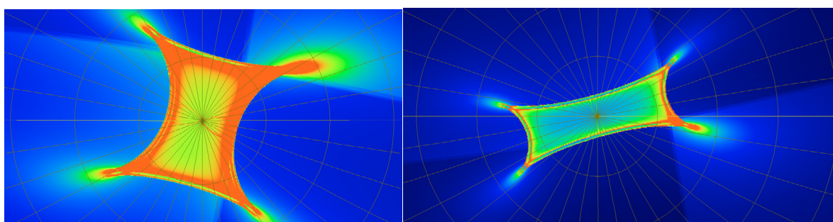
Fig. 15. Coverage map near the North ecliptic pole, achieved after 15 months of survey at 70 GHz ( left ) and 217 GHz ( right ), in units of integration time (blue to red color scale corresponds to 378/356 to 15 000 s/deg 2 for 70/217 GHz respectively). The horizontal extent of the maps is 63° at 70 GHz and 72° at 217 GHz (the angular separation between radial lines from the ecliptic pole is 10°). The figure illustrates how the shape of the highest integration areas narrows and rotates with frequency. Figures courtesy of ESA (X. Dupac).
