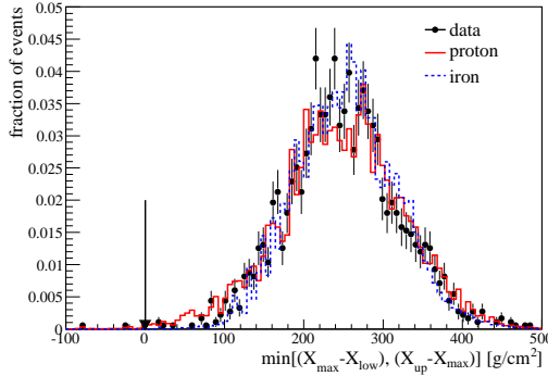
(e) distance of X_{max} to FOV boundary
