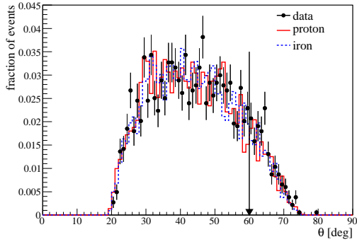
(c) zenith angle
