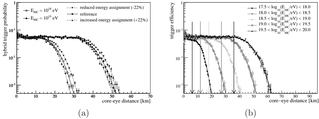
Fig. 7. The systematic uncertainty of the absolute energy scale of about 22 % would cause significant systematic uncertainties in the fiducial volume and the exposure (left panel). Dedicated event selection criteria are used to remove this dependency (right panel). The arrows show the cut values for the different energies based on eq. (10).
