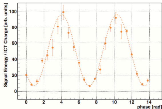
Figure 3: IPBSM Scan of tuned IP vertical beam, 310 +/- 30 (stat.) +/- 40 (syst.) nm
