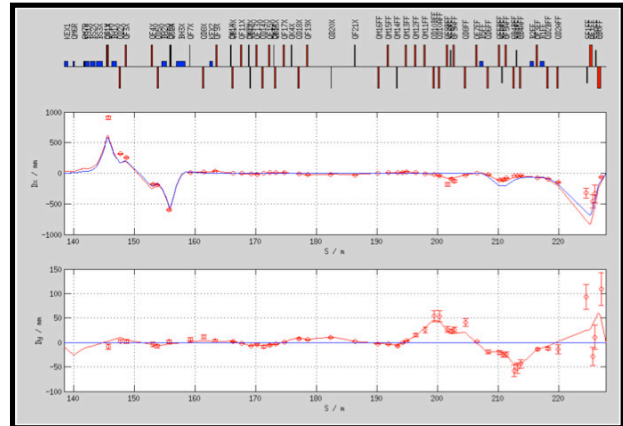
Figure 1: Dispersion measurements on EXT and FFS BPMs with model-based fit.
