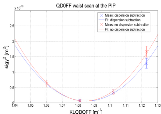
Figure 2: Vertical waist scan at IP using IPBSM and QDOFF.
