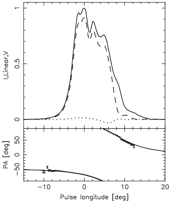
Figure 9. As in Figure 2, but for Parkes data of PSR J0742–2822 at 1369 MHz.
