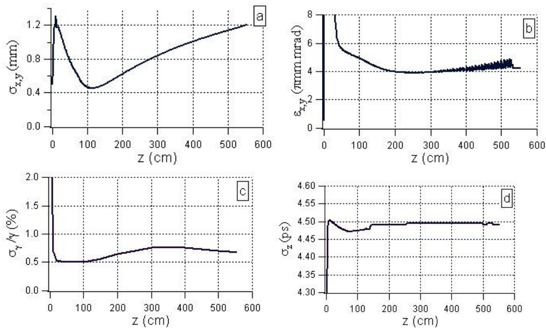
Figure 3 : results (r.m.s. values) of the PARMELA simulations for Q = 1 nC, 3000 macro-particles. Laser has a truncated Gaussian distribution: \sigma_t = 5 ps, T_{max} = 20 ps, \sigma_r = 6 mm, R_{max} = 1 mm. In a), transverse beam size; b), normalized emittance; c), energy spread; d), bunch length.
