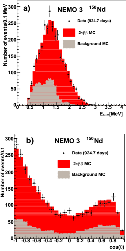
FIG. 3: (color online) Distributions of a) the energy sum of the two electrons, E_{\text{sum}} , and b) the angle between the two electrons, \cos \theta , for data compared to the sum of the background and 2\nu\beta\beta signal expectations.
