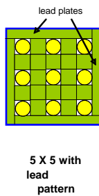
Fig. 1. Cross section of the FA pattern chosen for the VENUS-F core: fuel rodlets are cylindrical and lead ones are square.
