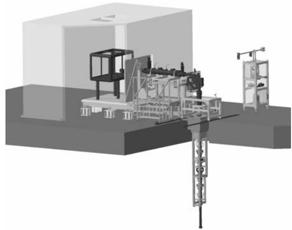
Fig.4. General layout of the GENEPI-3C machine with its supporting structures, Faraday cage and magnet cooling unit.
