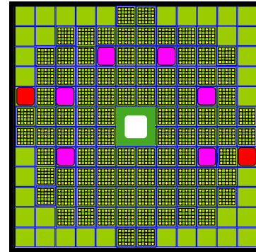
Fig. 8. SC1 core modified to be critical (100 FA's when SR up).
