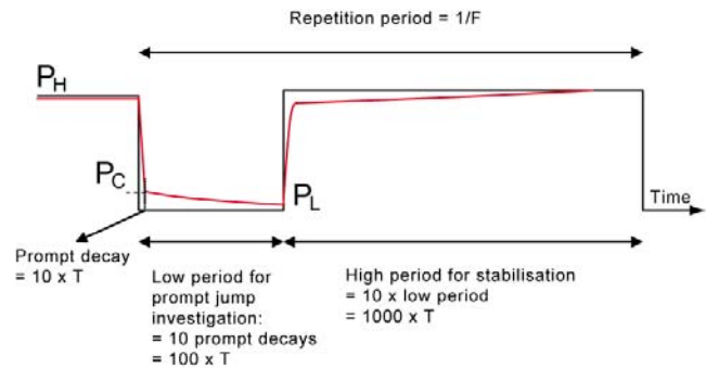
Fig. 10. Prompt jump technique principle (black: beam current, red: neutron flux).
