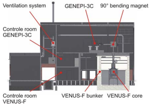
Fig. 3. Side view of the modified VENUS facility.
