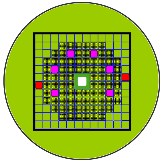
Fig. 2. Cross section (mid-plane) of the SC1 sub-critical core configuration (84 FA's).
