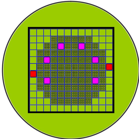
Fig. 6. Critical (CR0) configuration (88 FA's when SR up): safety (pink) and control (red) rod locations are shown.
