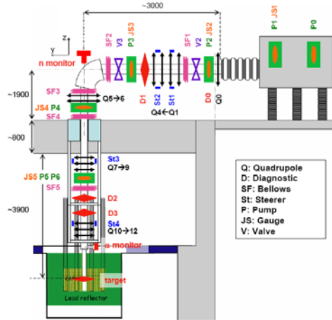
Fig. 5. Layout of the GENEPI-3C beam line components.
