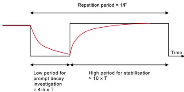
Fig. 9. Prompt decay fitting technique principle (black: beam current, red: neutron flux).
