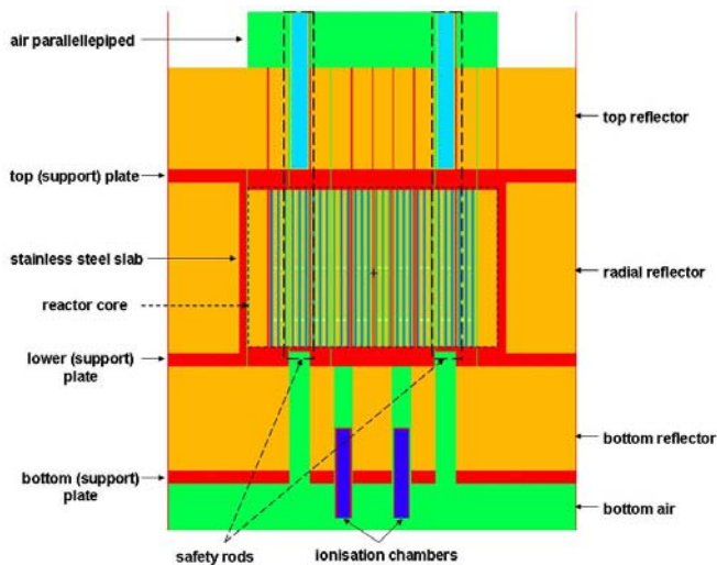
Fig.7. Critical (CR0) configuration vertical cut: all the rods up (legend: orange=lead, red=stainless steel, light blue=B 4 C, blue=ionization chambers, green=air, central orange/blue stripes=fuel).
