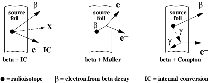
Fig. 2. Internal background production in the source foil.
