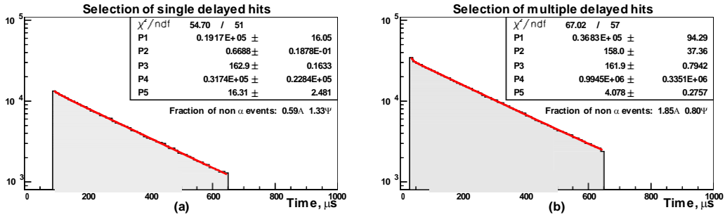
Fig. 6. The time distributions of events selected with (a) single and (b) multiple delayed signals. Each distribution was fit to the function: f(time) = P1 \cdot e^{-\frac{time}{P3/\ln 2}} + P2 + P4 \cdot e^{-\frac{time}{P5/\ln 2}} where P1 and P4 are scaling constants, P2 is the amplitude of random coincidences, P3 the ^{214}\text{Po} half-life in \mu\text{s} and P5 the time constant of the refirings.
