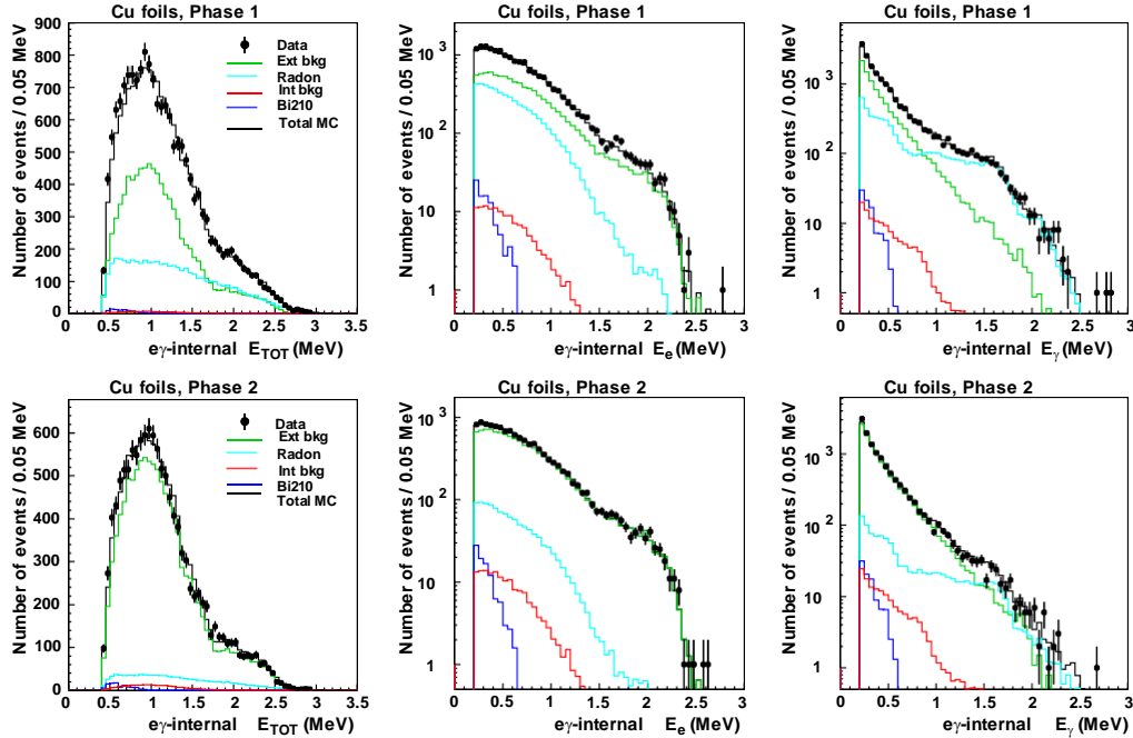
Fig. 22. The distribution of the energy sum of the e^- and \gamma -ray, the single e^- energy and the single \gamma -ray energy of internal e\gamma events from copper foils for Phase 1 and Phase 2 data.
