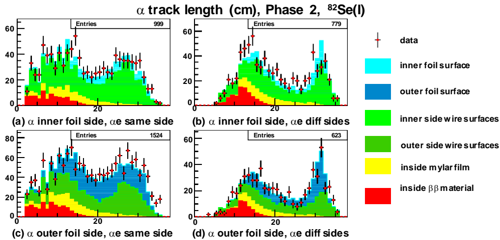
Fig. 20. Delayed track length distributions for the events of Phase 2 with vertices on the selenium source foils is shown by points with error bars. The MC simulations are shown with histograms. The results for events with both the \alpha track and the fast track ( e^- ) on the same side of the source foil are shown in plots (a) and (c) while those having the \alpha track and the electron on different foil sides are shown in plots (b) and (d).
