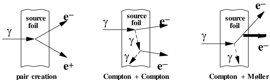
Fig. 3. External background production in the source foil.
