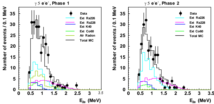
Fig. 19. Energy sum distribution of the two electrons in e\gamma -external events compared to the results obtained with the external background model.
